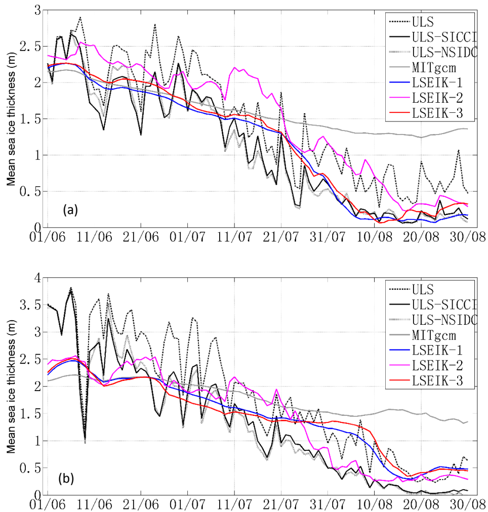
Figure xxx. Evolution of mean sea ice thickness (m) at (a) BGEP_2009A and (b) BGEP_2009D Beaufort Sea from 1 June to 30 August 2010. The black dotted lines show the original ULS thickness, the black solid and dashed lines show the obtained mean ice thickness using SICCI and NSIDC sea ice concentrations, respectively. The MITgcm free-run, LSEIK-1, LSEIK-2 and LSEIK-3 24 h ice thickness forecasts are shown as blue, magenta and red solid lines, respectively.
