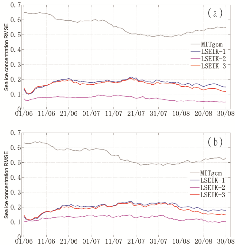
Figure 3. Temporal evolution of RMSE differences between sea ice concentration forecasts and the SICCI (a) and NSIDC (b) ice concentration data. The RMSE of the MITgcm free-run, LSEIK-1, LSEIK-2 and LSEIK-3 24-h forecasts are shown as gray, blue, magenta and red solid lines, respectively.
