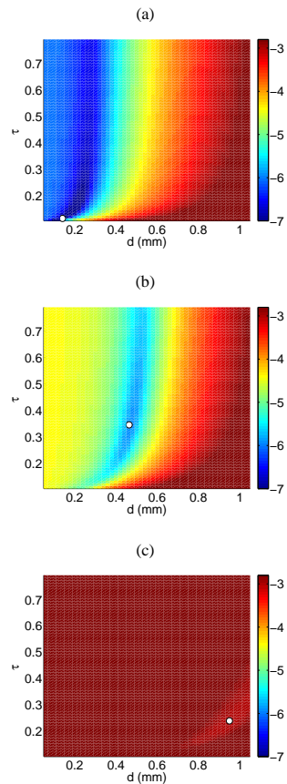
Figure 8. Contour plots for the “optimization landscape” for different snow types: colors show the log of the sum of the squared differences between measured and parametric SHS form \tilde{C}(k) as a function of (\tau, d) . (a) Precipitation particles. (b) Large rounded grains. (c) Depth hoar. The optimal values (\hat{d}, \hat{\tau}) for the respective sample are shown as white circles.
