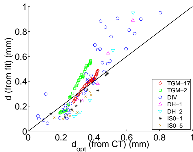
Figure 6. Scatter plot of the SHS diameter estimate \hat{d} and the optical diameter d_{opt} . The black solid line indicates the 1 : 1 relation.
