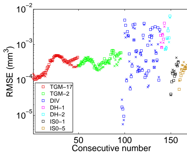
Figure 7. RMSE of the fit against the SHS model (squares) for all sub-series number in the entire data set. In addition we have shown the RMSE for the fit to the exponential model (crosses).
