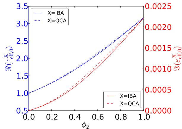
Figure 2. Real and imaginary parts of dielectric constant \epsilon_{\text{eff},0}^{\text{IBA}} and \epsilon_{\text{eff},0}^{\text{QCA}} in the very low frequency limit as a function of ice volume fraction \phi_2 .
