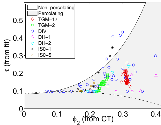
Figure 5. Estimated stickiness values \hat{\tau} as a function of ice volume fraction \phi_2 .
