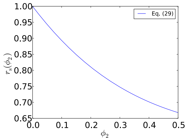
Figure 1. Ratio of scattering coefficient calculated with the IBA and DMRT theory as a function of ice volume fraction \phi_2 evaluated for \varepsilon_1 = 1 and \varepsilon_2 = 3.17 + 0.0022i .
