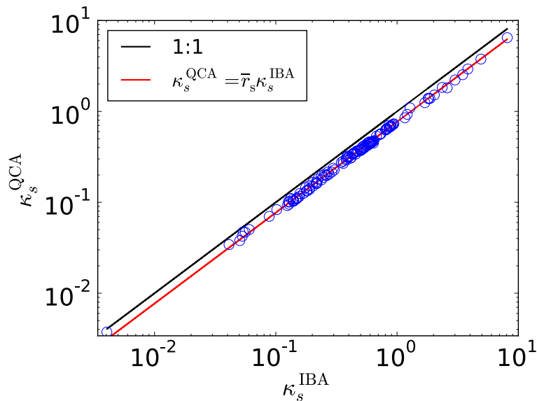
Figure 9. Scatter plot of the scattering coefficient of IBA and QCA-CP from Eqs. (28) and (22), respectively, evaluated for the optimal SHS parameters ( \hat{\tau} , \hat{\sigma} ) retrieved from the \mu CT images.
