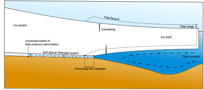
Figure 3. Schematic showing the various mechanisms by which tides can influence ice-stream flow. Note that grounding line migration, crevasse and tidal currents are not included in the model.
