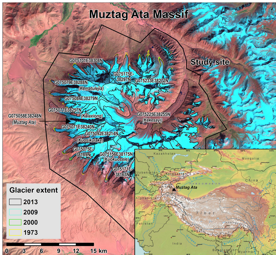
Figure 1. Overview of the Muztag Ata study site with investigated glaciers according to their ID in GLIMS (background image: Landsat 7 ETM+ of 11 September 2000).
