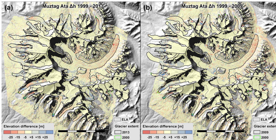
Figure 4. Co-registered difference images of 1999–2013 (a) and 1999–2009 (b) after outlier and gap-filling processing for glacier mass-balance and vertical uncertainty calculation.
