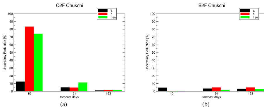
Figure 4. Uncertainty reduction for the Chukchi target area for flight transect C2F (panel a) and B2F (panel b) for target quantities mean ice concentration a , mean ice thickness h and mean snow depth hsn .
