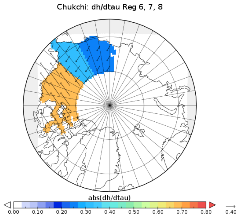
Figure 6. Wind stress direction with highest impact of tau component in control vector on ice thickness in Chukchi target region. Colour indicates magnitude.
