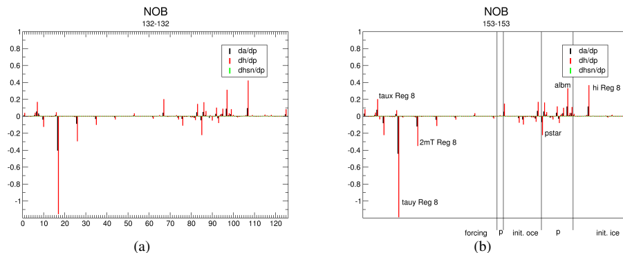
Figure 11. Sensitivity of target quantity over NOB area for 132 day (panel a), and 153 day (panel b) forecasts to 1 sigma prior uncertainty change in each control variable. Units of target quantities (and their sensitivities): ice concentration (a) (0–1); ice thickness ( h ) in m; snow thickness ( hsn ) in m.
