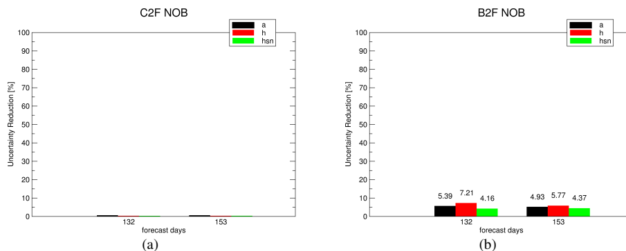
Figure 10. Uncertainty reduction for target areas NOB for flight transect C2F (panel a) and B2F (panel b).
