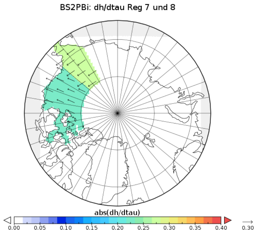
Figure 9. Wind stress direction with highest impact of tau component in control vector on ice thickness in BS2PB target region. Colour indicates magnitude.
