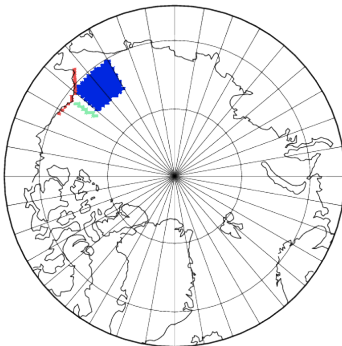
Figure 1. Target Regions: Chukchi (blue); North of Barrow (NOB, green) Bering Strait to Prudhoe Bay (BS2PB, red) .
