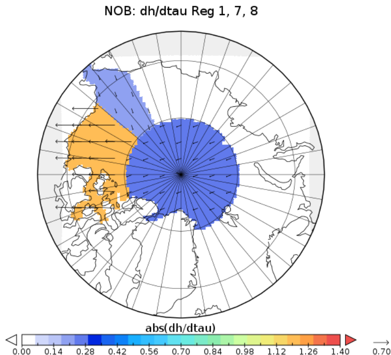
Figure 12. Wind stress direction with highest impact of tau component in control vector on ice thickness in NOB target region. Colour indicates magnitude.
