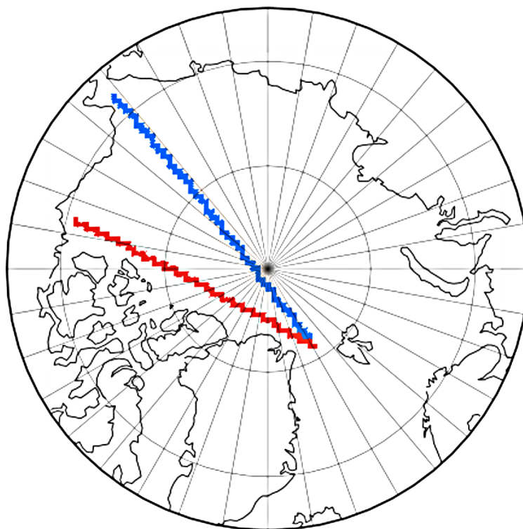
Figure 3. Flight transects: Chukchi to Fram (C2F, blue); Beaufort to Fram (B2F, red).
