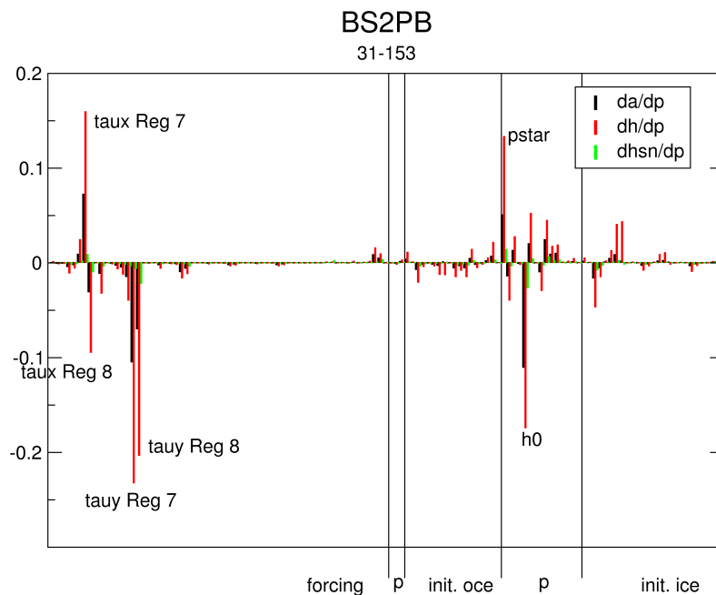
Figure 8. Sensitivity of target quantities for BS2PB area to 1 sigma prior uncertainty change in each control variable. Units of target quantities (and their sensitivities): ice concentration ( a ) (0–1); ice thickness ( h ) in m; snow thickness ( hsn ) in m.
