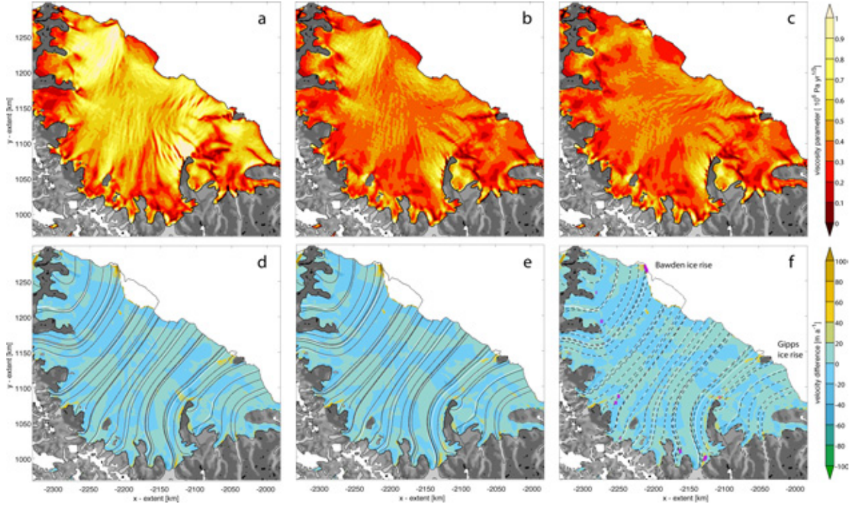
Fig. 3. Ice viscosity parameter (a–c) as inferred by the control method for the Larsen C ice shelf. Velocity difference (d–f) as in Fig. 1. (a, d) show results based on the actual Bedmap2 geometry, while (b, e) show results after flotation is guaranteed using the T-method. Inversion results on Larsen C for the T-geometry accounting for friction beneath pinning points not included in Bedmap2 (c, f). Gray shading indicates observed velocity magnitude on grounded parts of the ice sheet. The Bedmap2 shelf extents is indicated by a black contour line. On the shelf, black dashed and white lines indicate observed and modelled streamlines, respectively. The black dashed line on the grounded areas gives the 100 \text{ m a}^{-1} isoline of the observed surface velocities. Locations of pinning points (PIN5) not in Bedmap2 are indicated with pink squares in panel (e).
