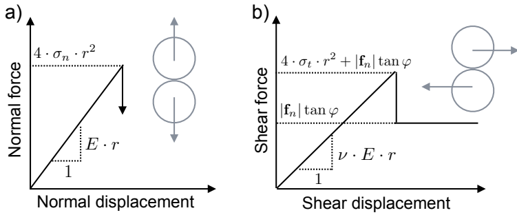
Figure 1: Behavior of a sphere-sphere contact in two simple cases: normal loading (a) and simple shearing under constant normal force \mathbf{f}_n (b).
