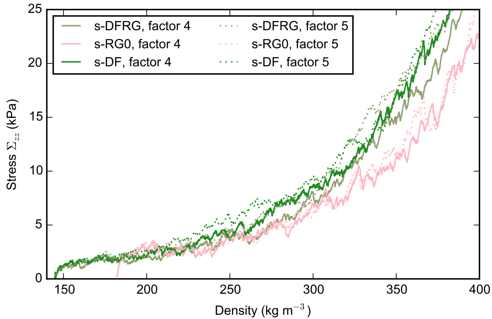
Figure 4: Simulated stress-density relation for the samples s-DF, s-DFRG and s-RG and two different factors (4 and 5) of resolution reduction.
