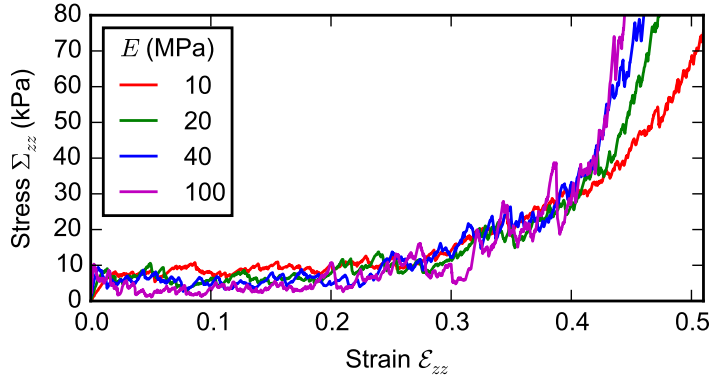
Figure 3: Computed stress-strain curves for different Young's moduli.
