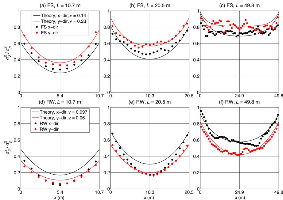
Figure 6. Comparison of the theoretical and sampled normalized squared error ( \sigma_z^2 / \sigma_p^2 ) for the case of a single measurement along a profile section of length L , as in Fig. 5a. The survey case applied to profiles in FS and RW along the x and y directions. Solid lines are the theoretical error using exponential decay exponents derived from the functions fitted to the sampled correlation functions of the two surfaces in the x and y directions.
