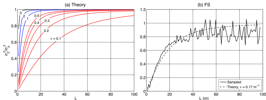
Figure 13. (a) Theoretical normalized squared error ( \sigma_z^2/\sigma_p^2 ) for the two-dimensional case with a single measurement in the middle of a square area with side dimension L . (b) Theoretical and sampled normalized squared error for the same two-dimensional survey applied to the snow depth field in FS. The dashed line is the theoretical error derived for an exponential decay exponent of 0.17 derived from the sampled correlation function of snow depth in FS, while the solid line is the sampled normalized squared error for the snow cover in FS.
