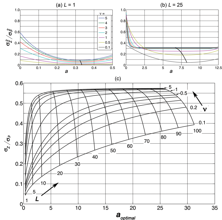
Figure 8. (a, b) Theoretical normalized squared error for the three-point pattern along a profile section in Fig. 5b, and for profile section lengths ( L ) of 1 (a) and 25 (b). Each of the colored lines corresponds to a specific decay exponent, \nu , and the black line marks the theoretical solution for a_{optimal} . (c) Theoretical normalized error and a_{optimal} for isolines of profile section lengths ( L ) and exponential decay exponents ( \nu ) for the three-point pattern along a profile section of length L in Fig. 5b.
