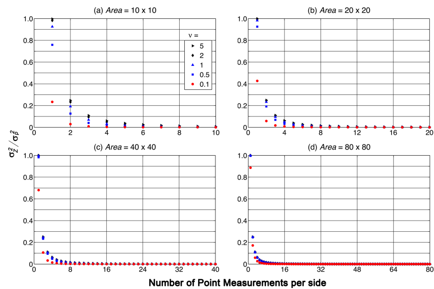
Figure 16. Theoretical normalized squared error ( \sigma_z^2 / \sigma_p^2 ) for the N by N point pattern in Fig. 12b, and for areas of side dimension ( L ) between 10 and 80. The exponential exponent is varied between 0.1 and 5.
