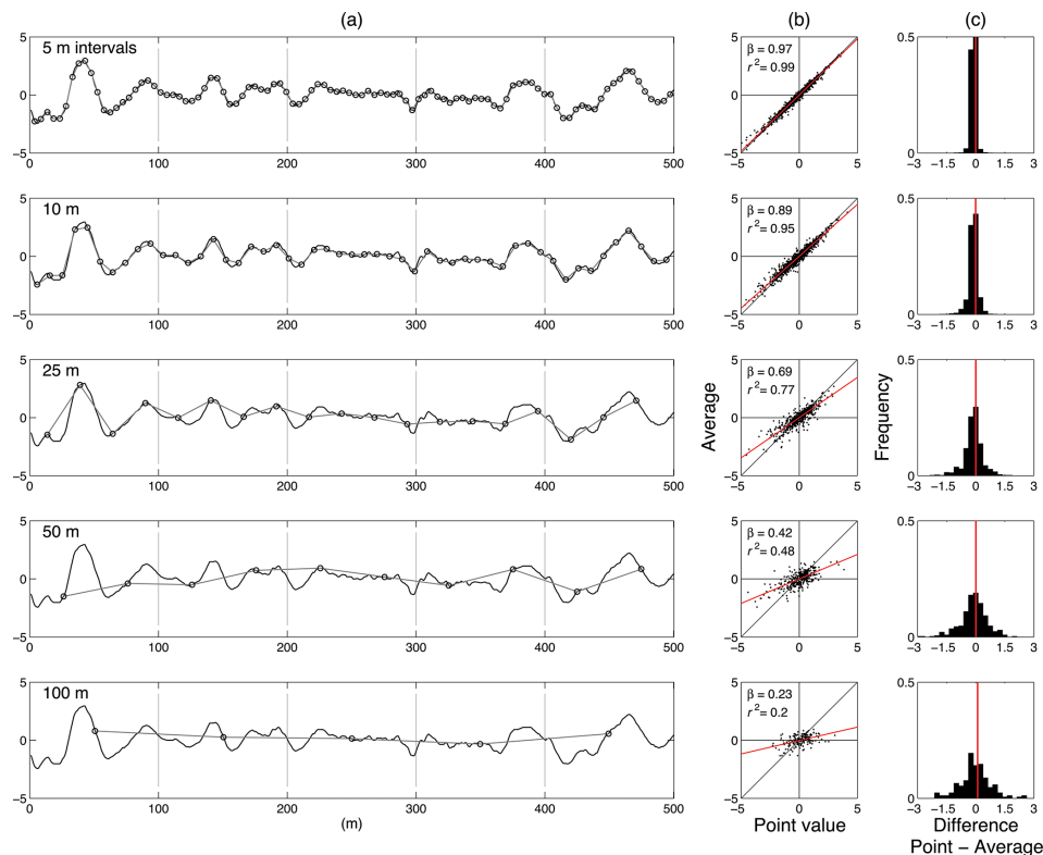
Figure 3. (a) As Fig. 2 but for an open and wind influenced environment at the Rabbit Ears – Walton Creek (RW) ISA of the CLPX (Trujillo et al., 2007; Cline et al., 2009). (b) Average values within sampling intervals (same as in a) vs. point samples for normalized snow depth profiles in the RW ISA. The red line is a linear regression fit, with slope \beta and r^2 as indicated in each plot. (c) Histograms of the difference between the point and average values for each of the sampling intervals. The vertical red line marks the mean difference.
