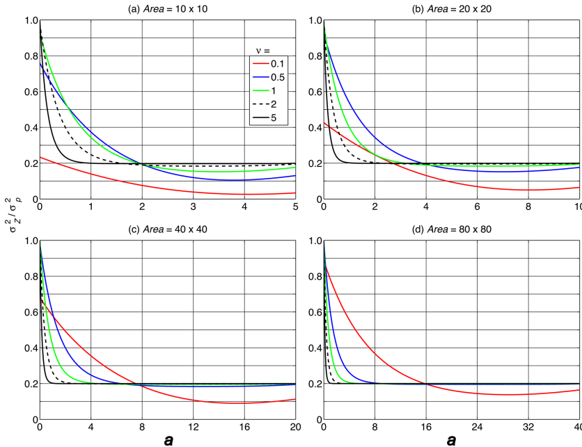
Figure 14. Theoretical normalized squared error ( \sigma_z^2/\sigma_p^2 ) as a function of the distance a from the center of the area for square areas of side dimensions ( L ) between 10 and 80. Each curve corresponds to an exponential decay ( \nu ) between 0.1 and 5.
