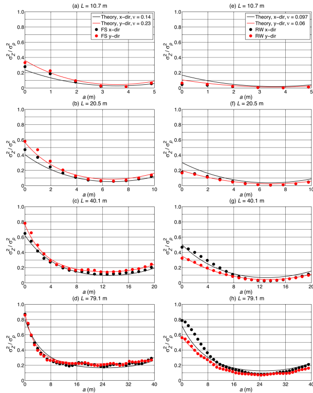
Figure 9. Theoretical and sampled normalized squared error ( \sigma_z^2 / \sigma_p^2 ) for the three-point pattern along a profile section in Fig. 5b, and for profile section lengths ( L ) between 10 and 80 m in FS and RW. The solid lines are the theoretical error from Eq. (8) using exponential decay exponents derived from the functions fitted to the sampled correlation functions of the two surfaces in the x and y directions, while the dots correspond to the sampled error for profiles in FS ( a–d ) and RW ( e–h ).
