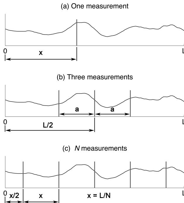
Figure 5. Survey designs for the sampling of a snow profile.
