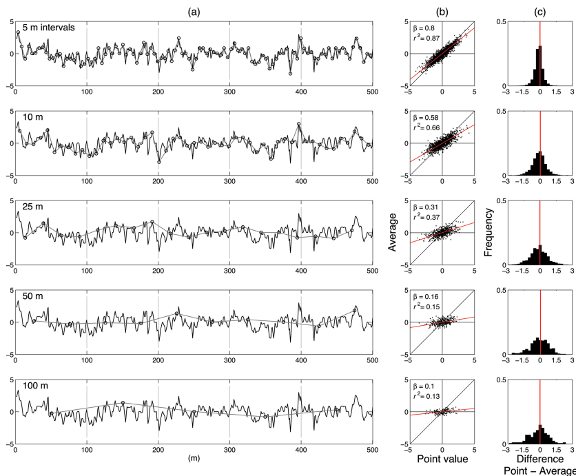
Figure 2. (a) Sample normalized snow depth profile (mean = 0, SD = 1) in a forested environment from LIDAR (1 m resolution) at the Fraser – St. Louis Creek (FS) intensive study area (ISA) of the Cold Land Processes eXperiment (CLPX) (Trujillo et al., 2007; Cline et al., 2009). The profile is sampled with regular separations (spacing) of 5, 10, 25, 50, and 100 m (from top to bottom, respectively). (b) Average values within sampling intervals (same as in a) vs. point samples for normalized snow depth profiles in the FS ISA. The red line is a linear regression fit, with slope \beta and r^2 as indicated in each plot. (c) Histograms of the difference between the point and average values for each of the sampling intervals. The vertical red line marks the mean difference.
