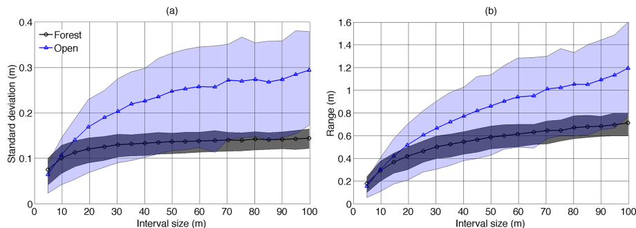
Figure 4. Sub-interval SD (a) and range (b) for varying interval lengths for profiles of snow depth in a forested environment (FS) and an open and wind-influenced environment (RW) in the Colorado Rocky Mountains (same regions as those in Figs. 2 and 3). The mean SD and mean range for the study areas are shown by the solid lines, while the shaded areas cover the quantiles between 25 and 75% of the values for all the intervals in these areas.
