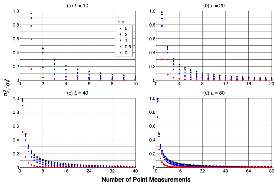
Figure 10. Theoretical normalized squared error ( \sigma_z^2/\sigma_p^2 ) for the N -point pattern along a profile section in Fig. 5c, and for profile section lengths ( L ) between 10 and 80 obtained from Eq. (10).
