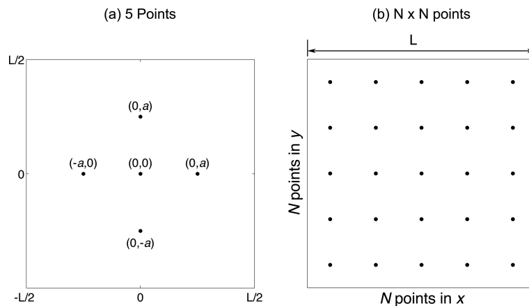
Figure 12. Sample survey designs with (a) a 5-point pattern centered in the area, and (b) a regularly spaced pattern. For the 5-point pattern, a can vary between 0 and L/2 , while for the N \times N points pattern, the separation between the measurements is determined by the number of points.
