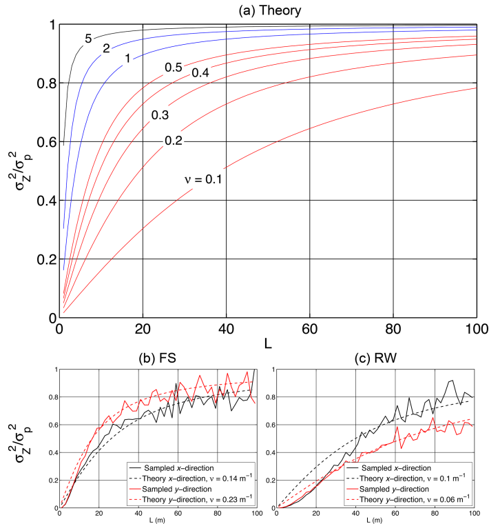
Figure 7. (a) Theoretical normalized squared error for a single measurement in the middle of a section of length, L , and for an exponential correlation function with a decay exponent, v . (b, c) Comparison of the theoretical and sampled normalized squared error for the same survey case applied to profiles in FS and RW along the x and y directions. Dashed lines are the theoretical error from Eq. (7) using exponential decay exponents derived from the functions fitted to the sampled correlation functions of the two surfaces in the x and y directions.
