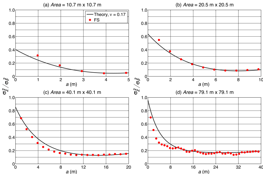
Figure 15. Theoretical and sampled normalized squared error ( \sigma_z^2 / \sigma_p^2 ) for the 5-point pattern in Fig. 12a over square areas of side dimensions ( L ) between 10.7 and 79.1 m. The separation distance a is varied from the center outwards. The solid line is the theoretical error derived for an exponential decay exponent of 0.17 derived from the sampled correlation function of snow depth in FS, while the solid red point markers are the sampled normalized squared error for the snow cover in FS.
