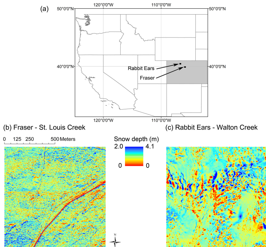
Figure 1. (a) Location of the Fraser and Rabbit Ears study areas in the state of Colorado (in grey). (b) LIDAR Snow depth distributions on 8 April 2003, at the Saint Louis Creek Intensive Study Area (ISA) and (c) on 9 April at the Rabbit Ears ISA.
