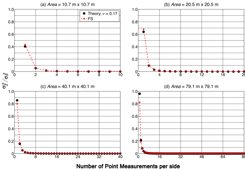
Figure 17. Theoretical and sampled normalized squared error ( \sigma_z^2 / \sigma_p^2 ) for the N by N point pattern in Fig. 12b, and over square areas of side dimensions ( L ) between 10.7 and 79.1 m. The solid black point markers are the theoretical error for an exponential decay exponent of 0.17 derived from the sampled correlogram of snow depth in FS. The dotted red lines with circle markers are the sampled normalized squared error for the snow cover in FS.
