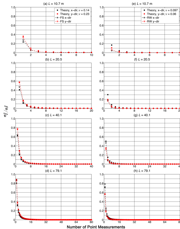
Figure 11. Theoretical and sampled normalized squared error ( \sigma_z^2 / \sigma_p^2 ) for the N -point pattern along a profile section in Fig. 5c, and for profile section lengths ( L ) between 10 and 80 m in FS and RW. The solid point markers are the theoretical error from Eq. (10) using exponential decay exponents derived from the functions fitted to the sampled correlograms of the two surfaces in the x and y directions, while the circle markers with the dotted lines correspond to the sampled error for profiles in FS (a–d) and RW (e–h).
