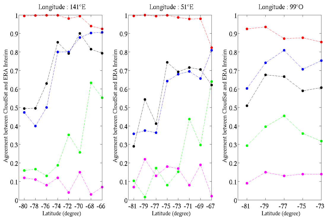
Figure 1 : the same figure than the figure 5 in the discussion paper but with a threshold adjusted to maximize the Heidke skill score at every locations. The pink curve is the value of the threshold determined to maximize the Heidke skill score. Red curve : proportion of flags indicating periods without precipitation that match with periods without precipitation in ERA Interim. Blue curve : proportion of flags indicating precipitation certain that match with precipitation events in ERA Interim. Green curve proportion of flags indicating precipitation possible that match with precipitation events in ERA Interim. Black curve : Heidke skill score assessed using flags indicating precipitation certain and period without precipitation.
