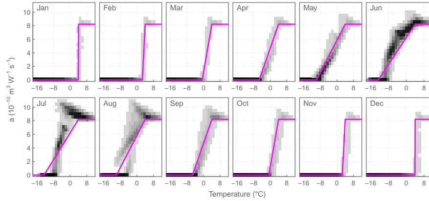
Fig. 3. Monthly diagnostic values of the coefficient a versus temperature (shading represents density of points), along with the parameterization given by Eq. 6 (magenta line).
