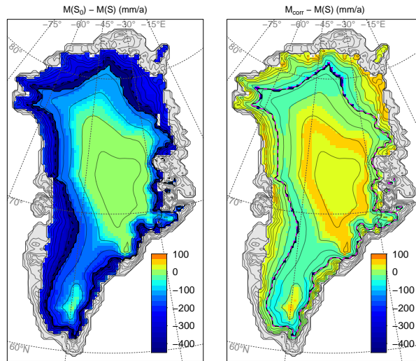
Fig. 6. Error in melt (mm/a) for a 3^{\circ}\text{C} summer temperature anomaly at 126 ka BP calculated with the reduced ( left ) and insolation-corrected ( right ) model, compared to melt from the full model. The solid and dashed black lines in the left panel show the equilibrium line altitudes for the full ( M(S) ) and reduced model ( M(S_0) ), respectively. The dashed magenta line in the right panel shows the same for the insolation corrected-model.
