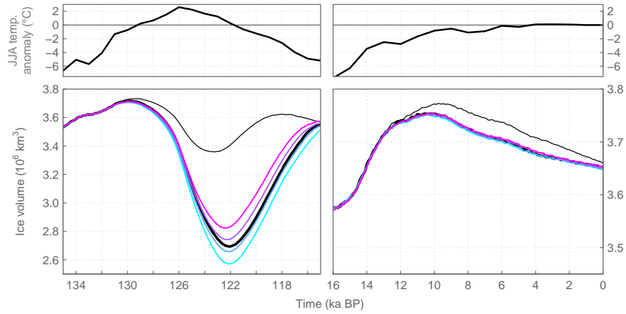
Fig. 7. Transient simulations of the Eemian ( left ) and the Holocene ( right ) with a fully coupled climate–ice sheet model. Top: Applied summer temperature anomaly forcing. Bottom: Ice volume from simulations in which melt is calculated with the full model (thick black line), the reduced model forced with present-day insolation (thin black line) and an ensemble of insolation-corrected model versions with the parameter T_{\min} set to -15 , -14 , -13 and -12^{\circ}\text{C} (cyan to magenta lines, respectively).
