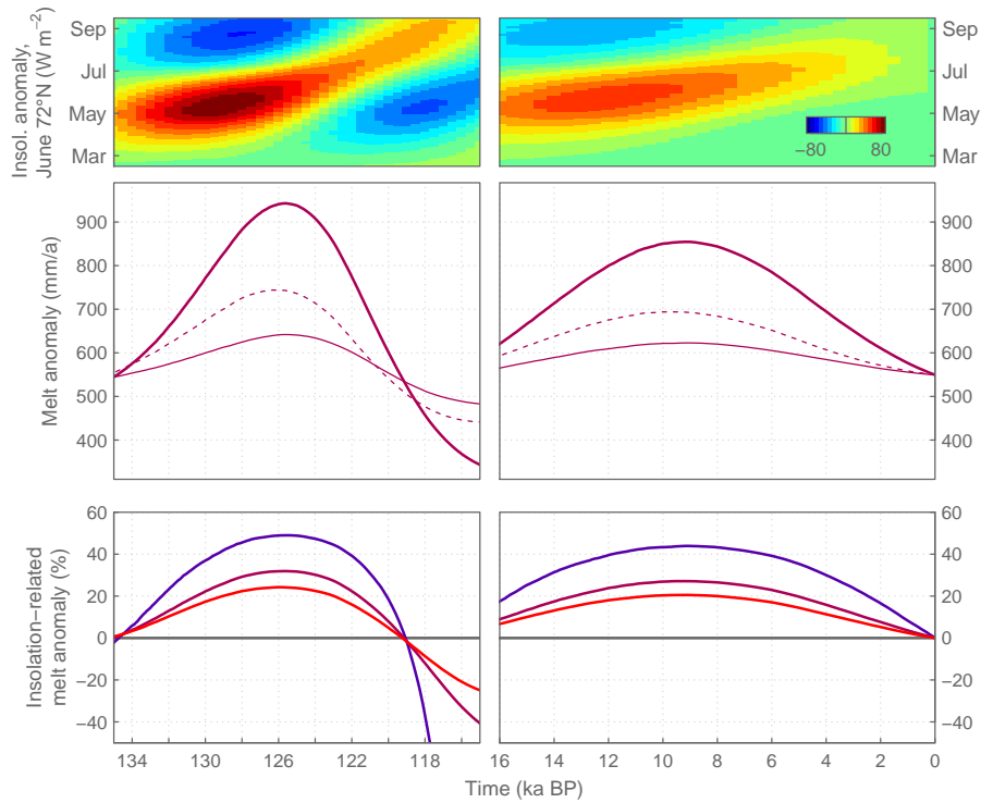
Fig. 1. Melt anomalies relative to present day for the Eemian ( left ) and the Holocene ( right ). Top: Representative insolation anomaly at 72^\circ\text{N} for summer months (Mar-Sep). Middle: Melt anomalies given a constant JJA temperature anomaly of 3^\circ\text{C} calculated from the full model (thick line), the reduced model (thin line) and the reduced model using surface conditions from the full model (dashed line). Bottom: Percentage of the melt anomaly due to changes in insolation for constant summer temperature anomalies of 1^\circ\text{C} , 3^\circ\text{C} and 5^\circ\text{C} (blue, purple and red, respectively).
