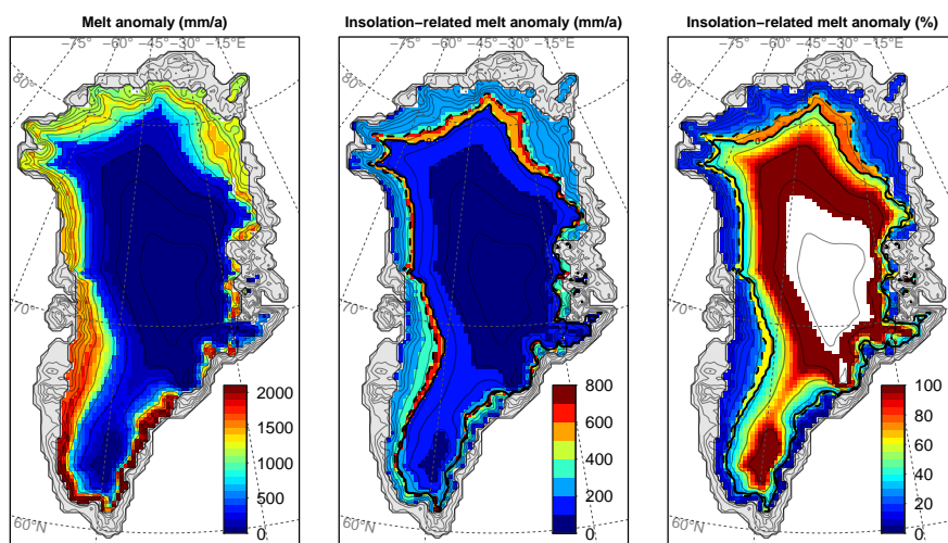
Fig. 2. Melt anomaly at 126 ka BP given a 3^{\circ}\text{C} summer temperature anomaly relative to today. Left: Total melt anomaly (mm/a). Center: Melt anomaly (mm/a) due to insolation changes. Right: Percentage of melt due to insolation changes. In the center and right panels, the solid and dashed black lines show the equilibrium line altitude for the full ( M(S) ) and reduced model ( M(S_0) ), respectively.
