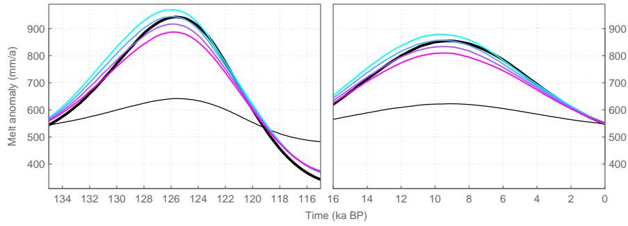
Fig. 5. Greenland ice sheet melt anomalies for the Eemian ( left ) and the Holocene ( right ) given a 3^{\circ}\text{C} summer temperature anomaly relative to today, calculated with the full model ( M(S) , thick black line), the reduced model ( M(S_0) thin black line) and an ensemble of insolation-corrected model versions ( M(S_0)_{\text{corr}} ) with the parameter T_{\text{min}} set to -15 , -14 , -13 and -12^{\circ}\text{C} (cyan to magenta lines, respectively).
