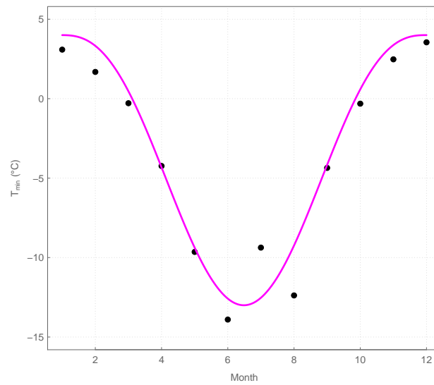
Fig. 4. Seasonal value of T_{\min} estimated from a linear fit to the diagnostic values of a in the range of 0 < a < a_{\max} (black points) and compared to the parameterization given by Eq. 7 (magenta line)
