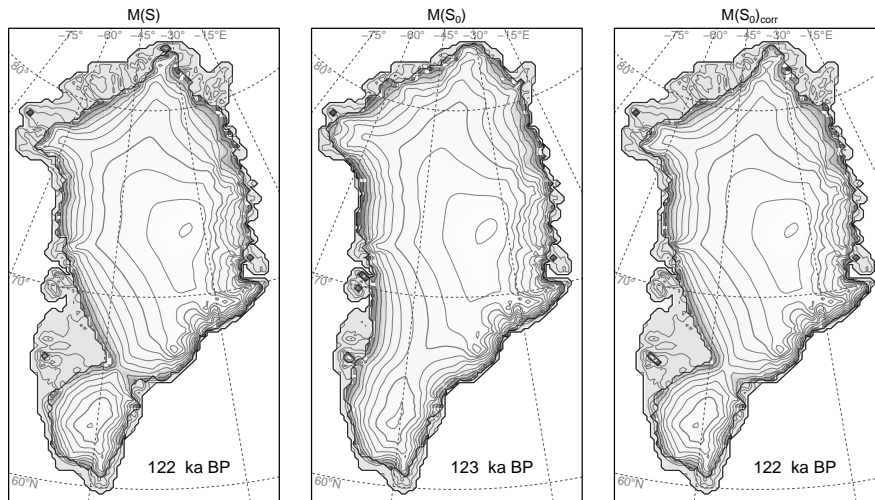
Fig. 8. Distribution and timing of the minimum ice sheet volume during the Eemian for coupled simulations using the full model ( left ), the reduced model ( middle ) and the insolation-corrected model ( right ).
