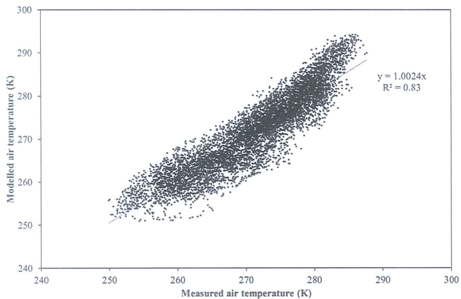
Fig. 2. Hourly temperatures recorded by the AWS1 Forni ( T_{AWS} ) during 2010 ( x axis) vs. the modelled ones ( T_B , y axis) derived from Bormio data shifted to the AWS1 Forni elevation through the application of the mean tropospheric lapse rate.
