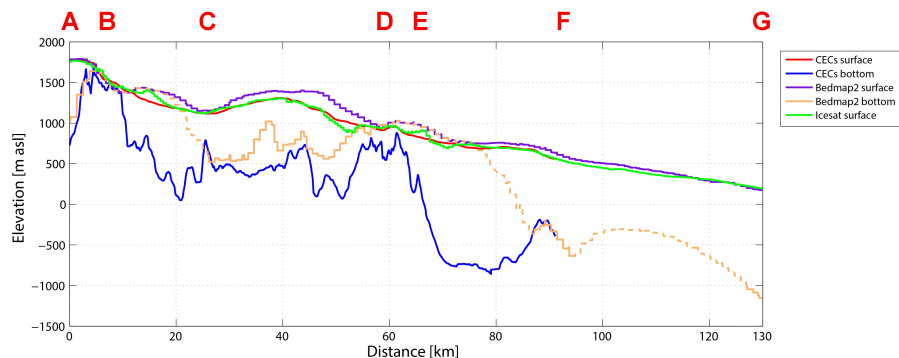
Fig. 9. Comparisons of surface and bedrock topography of different data sources along transect A–G (see Fig. 1 upper for location of transect). CECs surface and bedrock from year 2010. IceSat surface from 2003–2005, Bedmap 2 surface and Bedrock from Fretwell et al. (2013). Bedmap2 bottom dashed line is interpolated.
