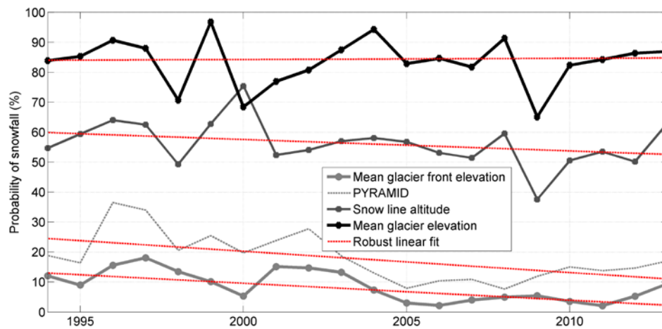
1442 Figure 9. Trend analysis of annual probability of snowfall on total cumulated 1443 precipitation. The red lines represents the robust linear fitting of the time series 1444 characterized by the associated Sen's slope (more details in the caption of Fig. 3).
