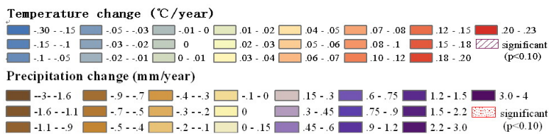
Fig. 1. Figure 9 Temperature (upper) and precipitation (lower) changes during the period 1979/80-2010/11 in the northern hemisphere. The precipitation change only use the grids which have continuous precipita
