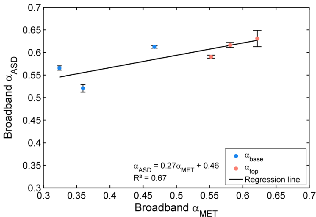
Figure 4. Broadband \alpha_{base} (blue dots) and \alpha_{top} (pink dots) vs. \alpha_{ASD} and \alpha_{MET} (i.e., both \alpha_{base} and \alpha_{top} ) measurements fitted to a linear regression equation ( R^2 = 0.67 ). The value of \alpha_{ASD} error is based on the standard deviation of individual \alpha_{ASD} measurements.
