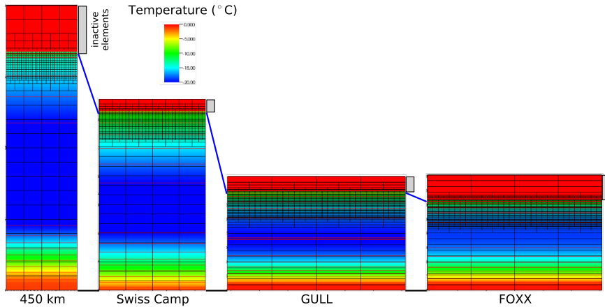
Figure 4. The gradual deformation of the computing mesh along the flow line to accommodate for the varying ice thickness. The ice surface is marked with blue lines between meshes, and inactive elements are indicated with gray bars (red elements on top). The precise position of the surface with respect to the mesh is tracked with adaptive mesh refinement. Modeled ice temperatures are indicated with colors. The greenish elements close to the surface are accumulated during flow (thickest at Swiss Camp at the equilibrium line) and slowly removed from the top due to ablation (sites GULL and FOXX). Note that computational mesh shown is for illustration only, actual model runs were performed on considerably finer meshes.
