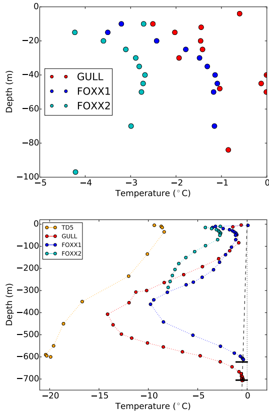
Figure 2. Measured ice temperatures. (a) shows near-surface temperatures at sites GULL and FOXX. Holes FOXX1 and FOXX2 are 86 m apart. (b) shows measured ice temperatures in four boreholes at the drill sites TD5 (Swiss Camp; data from Thomsen et al., 1991), GULL and FOXX. The dashed line indicates the pressure melting temperature.
