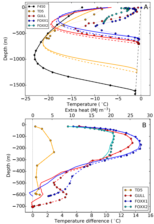
Figure 5. Measured and modeled temperatures at the three sites Swiss Camp (TD5), GULL and FOXX. Dots Symbols connected by dotted lines indicate measurements. Dashed lines refer to the reference model run mD (dissipation only). Solid lines refer to run mE (additional heat sources from enhanced shear straining in ice-age ice). The scale on top of the lower panel shows the extra heat per volume with respect to model run mD (dissipation only).
