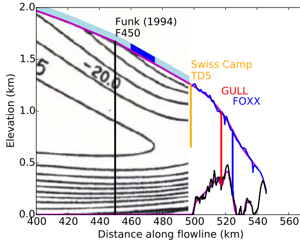
Figure 3. The locations and depths of temperature profiles at sites TD5, GULL and FOXX are shown as colored vertical lines on a background plot of the modeled temperature field from Fig. 7b in Funk et al. (1994). The temperature profile F450 at horizontal coordinate 450 km is used as model input. Bedrock (black) and surface (blue) was obtained from detailed radar data ( DTU Space and Remote Sensing, 2005 ) ( Gogineni, 2012 ). Smoothed versions, indicated with purple lines, were used as model input. The light-blue area indicates cold firn conditions, and the dark blue area between 460 and 475 km the area of within which the temperate firn conditions that emerges at TD5 was accumulated between 1570-1730.
