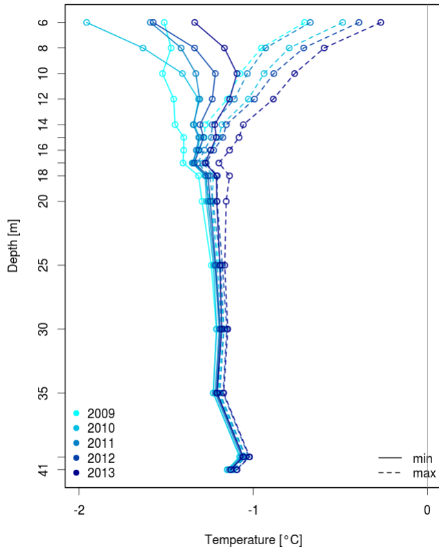
Figure 7. Minimum (solid lines) and maximum (dashed lines) temperature profiles in the borehole DP below 6m of depth.
