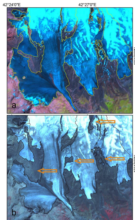
Fig. 5. Expansion of exposed rocks on the southern slope of Mt. Elbus: (a) 1999 and (b) 2012. Arrows point at the expanded areas of exposed rocks. The 1999 Landsat ETM+ image (Table 1) is used as background.
