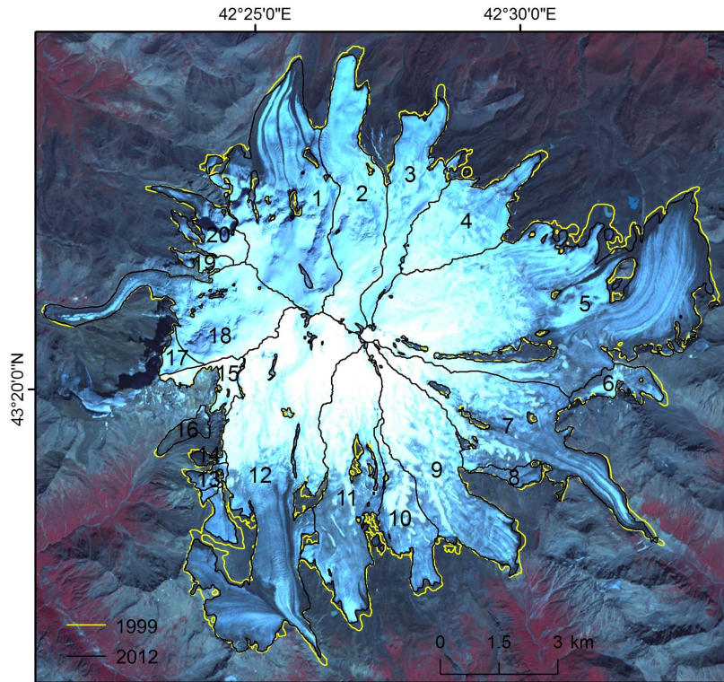
Fig. 4. Changes in glacierised area of Mt. Elbus between 1999 and 2012. See Table 4 for the statistics of changes in areas of individual glaciers. The 1999 Landsat ETM+ image (Table 1) is used as background.
