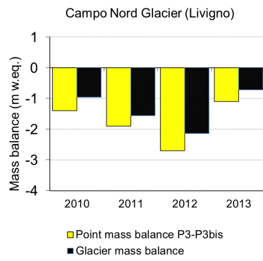
Figure 1. Campo Nord: Glacier vs Point mass balance (2010-2013).
