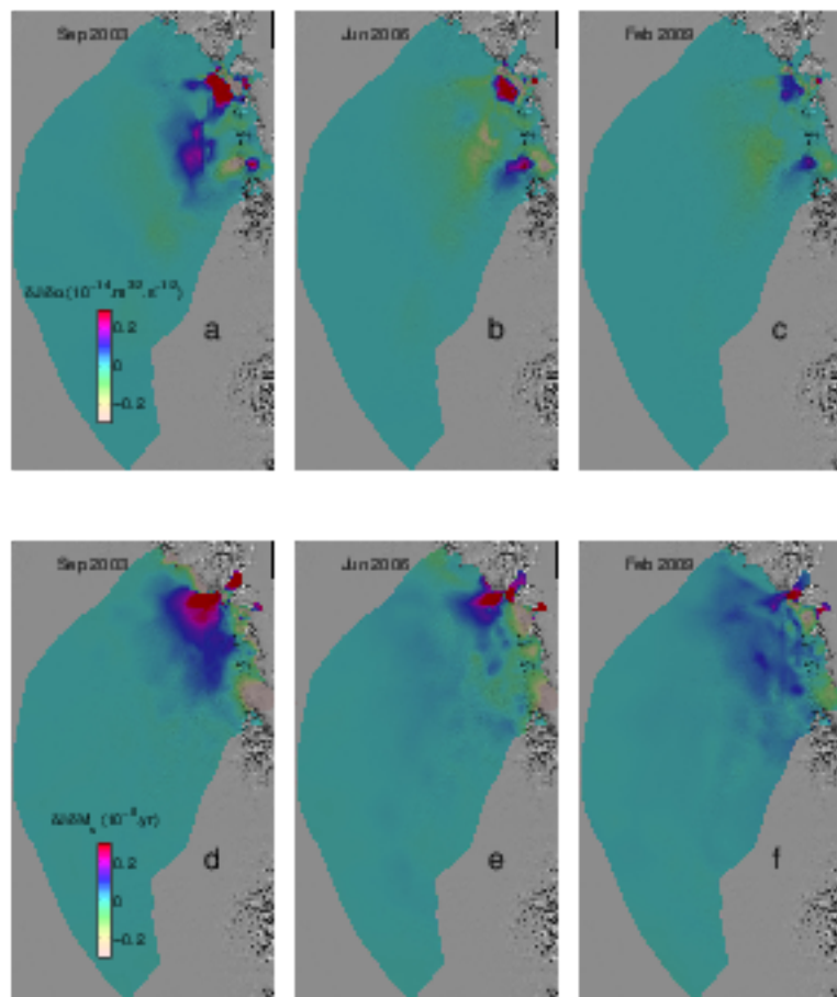
Fig. 5. a), b) and c): gradients \partial J/\partial\alpha ( m^{3/2}\cdot s^{-1/2} ) of the cost function J with respect to the ice/bed friction coefficient \alpha in respectively, September 2003, June 2006 and February 2009. d), e) and f): gradients \partial J/\partial M_s (yr) of the cost function J with respect to the surface mass balance M_s in respectively, September 2003, June 2006 and February 2009.
