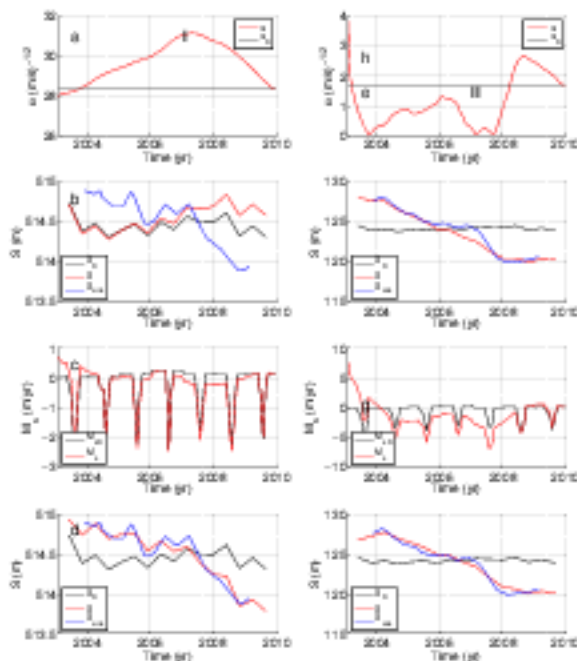
Fig. 7. Improvement in the best-fit between modeled surface height compared to and the altimetry record after inversion of basal friction \alpha and surface mass balance M_s for the two locations indicated in Fig.(3f) corresponding to the center of 79 North (frames a),b),c) and d)) and a location near the grounding line of Zacharise Zacharig Isstrøm (frames (e), f), g) and h)). Frames a) and e) show the difference between the original time series \alpha_0 of friction (in black), and the inverted one \alpha (in red). Frames b) and f) show the improvement in the modeled surface height (in red) best-fit to observations (in blue) compared to the original model (in black) and the better fit to observations (in blue) . Frames c) and g), d) and h) show similar results as for a) and e) and b) and f), with surface mass balance M_s being the quantity inverted for instead of \alpha . Errors in observed surface height time series for locations I and II, which are below the ELA, depend on the SERAC processing only (ice is assumed fully dense, with no firn compaction involved), and are estimated respectively at 8 cm and 1.2 m.
