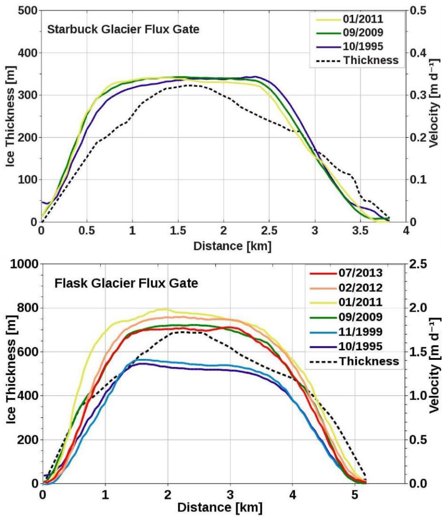
630 Fig. 7. Ice thickness and surface velocity across the flux gate of Starbuck Glacier (top) and Flask 631 Glacier (bottom). Ice thickness from Farinotti et al. (2013; 2014).
