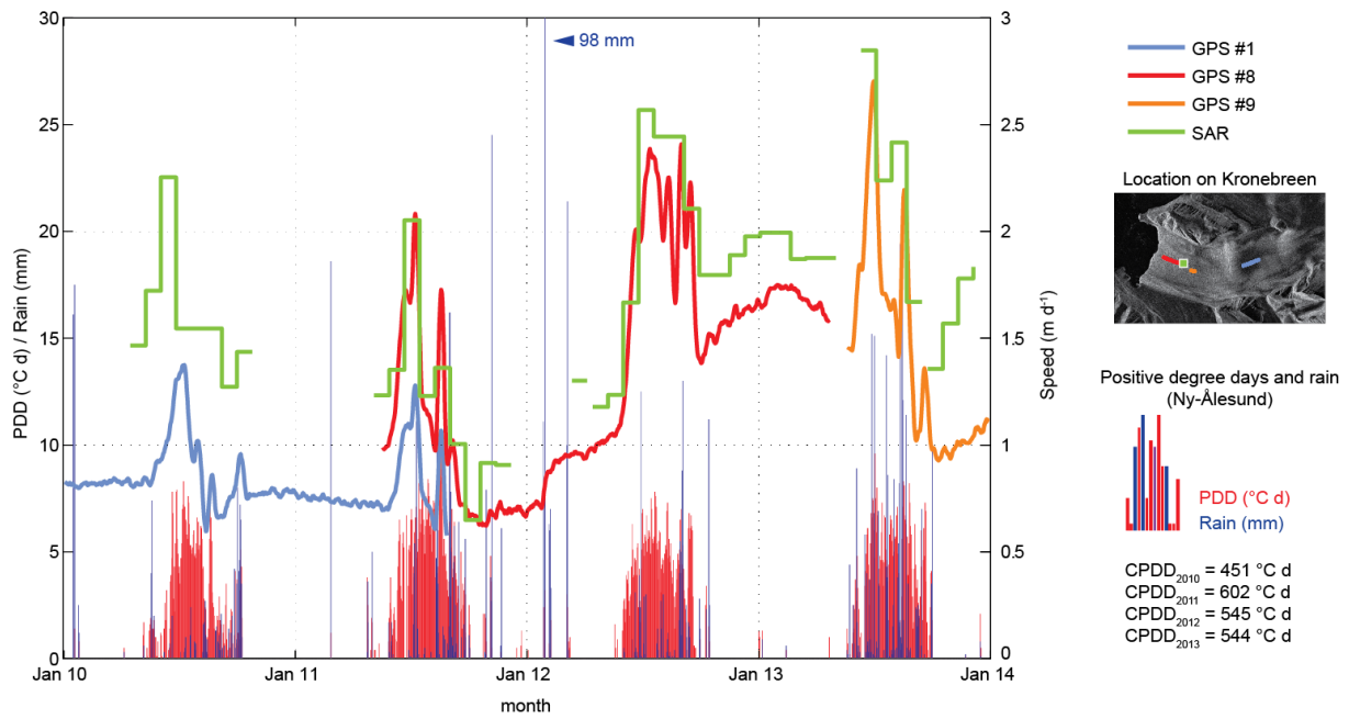
1 2 Fig. 6 Time series of speed of Kronebreen between 2010 and 2013 linked to water supply by 3 melt (positive degree days (°C) and rain events (mm) from weather station in Ny-Ålesund). 4 Speed of Kronebreen ( \text{m d}^{-1} ) derived from RS-2 (green) and GPS (blue/red/orange).
