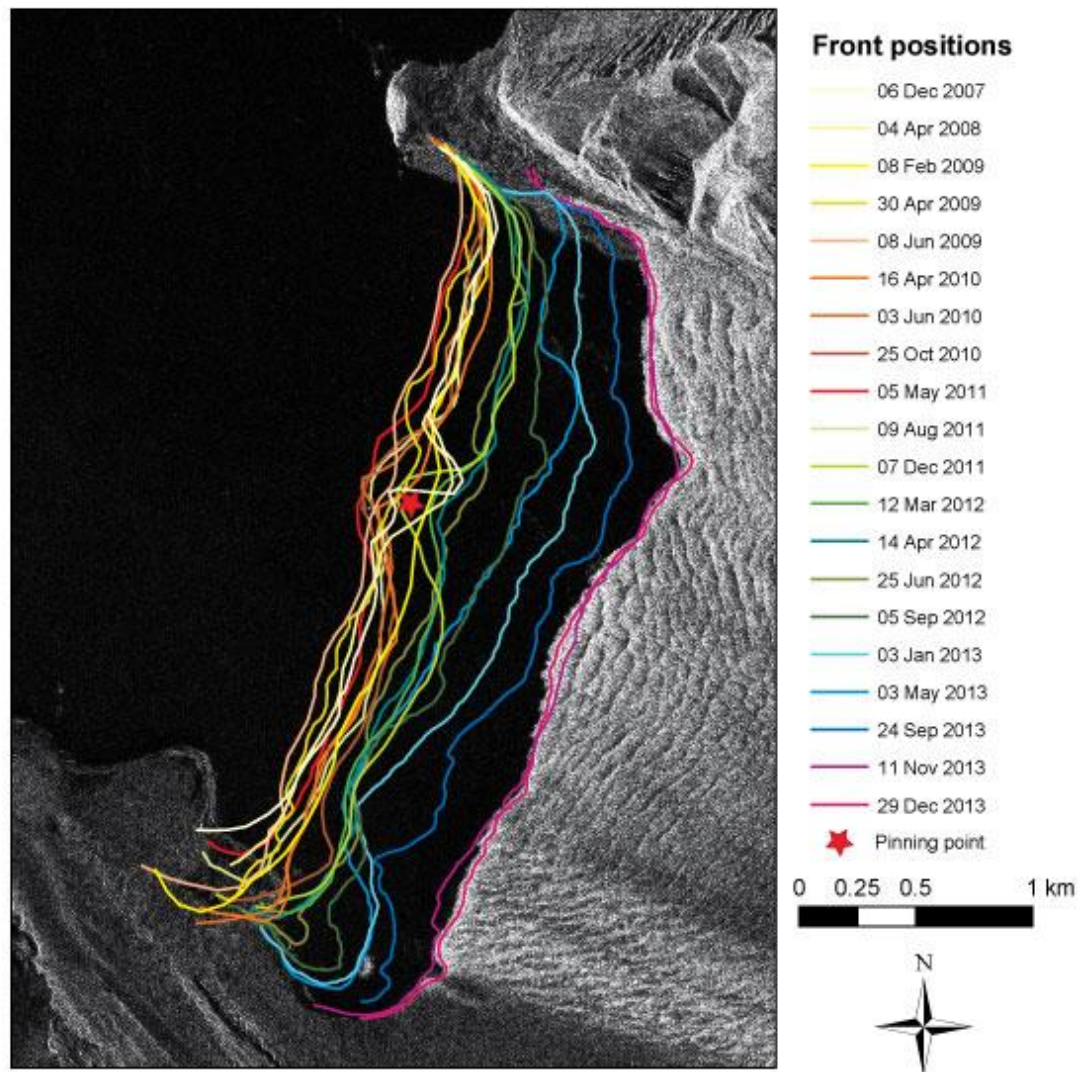
1 2 Fig. 7 Selected calving front positions of Kronebreen between December 2007 and December 3 2013. Background image RS-2 UF of 29 December 2013.
