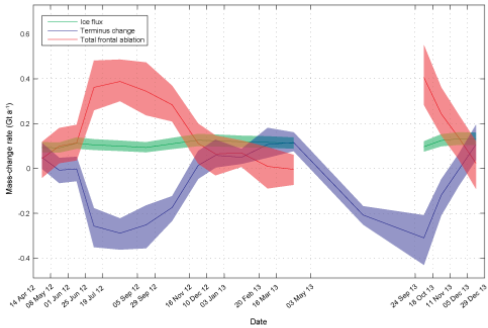
Fig. 12 Frontal ablation of Kongsbreen between 14 April 2012 and 29 December 2013 and components, ice flux and terminus position changes. Note that the ice flux could not be estimated between May and September 2013 and therefore set to 0.0 Gt a -1 as the quality of the speed map was not sufficient to extract glacier speed along the fluxgate.
