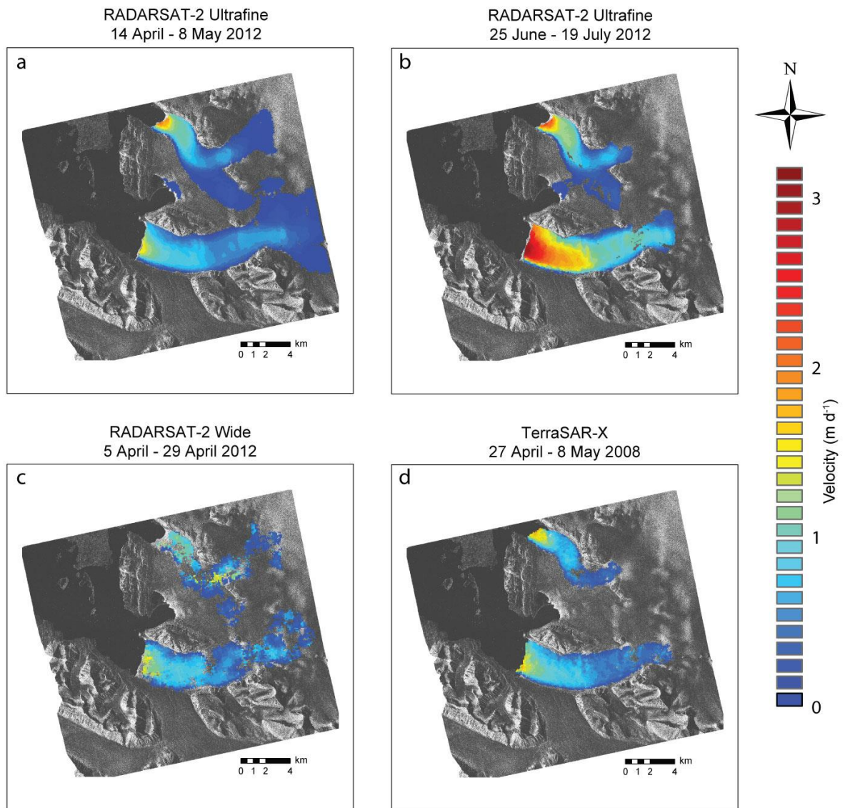
1 2 Fig. 2 Selected speed fields of Kronebreen and Kongsbreen from SAR feature tracking. (a) 3 RS-2 UF 14 April 2012-08 May 2012 (b) RS-2 UF 25 June 2012-19 July 2012 (c) RS-2 W 05 4 April 2012-29 April 2012 (d) TSX 27 April 2008 – 08 May 2008.
