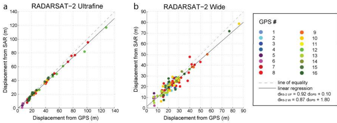
1 2 Fig. 3 Validation of glacier displacement: Displacements extracted from SAR maps at the 3 position of GPSs and plotted against GPS displacements (a) RS-2 UF vs. GPS (b) RS-2 W vs. 4 GPS.
