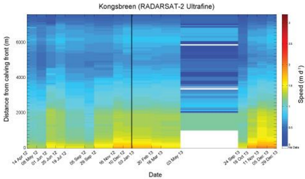
1 2 Fig. 9 Time series of speed along centerline of Kongsbreen (Fig. 1) between 14 April 2012 3 and 29 December 2013 based on RS-2 UF data. Note the reduced quality of matching results 4 and missing matches at the calving front between 03 May 2013 and 24 September 2013 due to 5 the long time interval between acquisitions.
