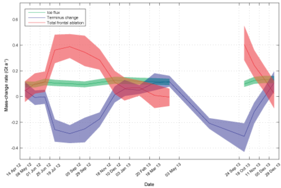
Fig. 8 Frontal ablation of Kronebreen between 14 April 2012 and 29 December 2013 and components, ice flux and terminus position changes. Note that the ice flux could not be estimated between May and September 2013 and therefore set to 0.0 Gt a -1 as the quality of the speed map was not sufficient to extract glacier speed along the fluxgate.
