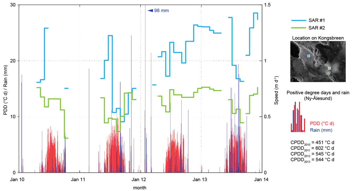
Fig. 10 Time series of speed of Kongsbreen between 2010 and 2013 linked to water supply to the bed by melt and rain (positive degree days ( ^{\circ}\text{C} ) and rain events (mm) from weather station in Ny-Ålesund). Speed at two points of Kongsbreen ( \text{m d}^{-1} ) from RS-2 UF and RS-2 W (see inset).
