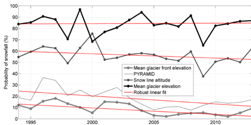
1517 Figure 9. Trend analysis of annual probability of snowfall on total cumulated 1518 precipitation. The red lines represents the robust linear fitting of the time series 1519 characterized by the associated Sen's slope (more details in the caption of Fig. 3).
