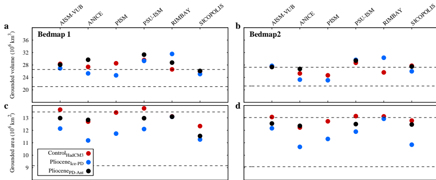
Fig. 12. Final grounded ice volume ( 10^6 \text{ km}^3 ) and grounded ice area ( 10^6 \text{ km}^2 ) for the six models. a) Grounded ice volume with Bedmap1. b) Grounded ice volume with Bedmap2. c) Grounded ice area with Bedmap1, and d) Grounded ice area with Bedmap2. Control HadCm3 in red, Pliocene Ice-PD in blue and Pliocene PD-Ant in black. The horizontal dashed lines indicate the PD and Pliocene grounded ice volume and ice area of the initial ice-sheet topographies with Bedmap1 (a,c) and Bedmap2 (b,d).
