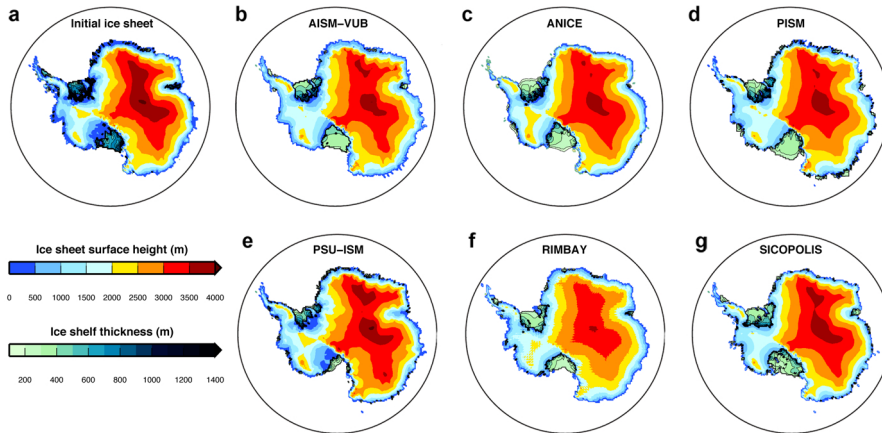
Fig. 3. Ice surface topography and thickness of the ice shelves for the Control HadCM3 simulation, with HadCM3 climate forcing. a) Initial ice sheet from Bedmap1, b) AISM, c) ANICE, d) PISM, e) PSU-ISM, f) RIMBAY, g) SICOPOLIS.
