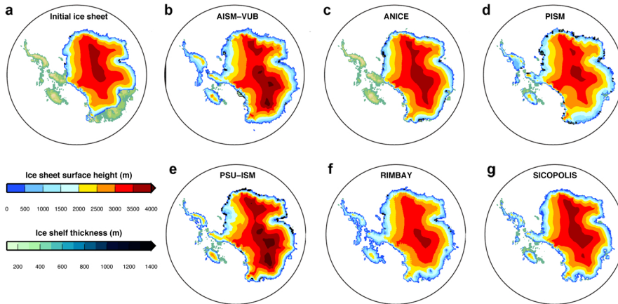
Fig. 6. Ice surface topography and thickness of the ice shelves for the Pliocene Ice-PRISM3 simulation, with HadCM3 Pliocene climate forcing. a) Initial PRISM3 ice sheet with Bedmap1, b) AISM, c) ANICE, d) PISM, e) PSU-ISM, f) RIMBAY, g) SICOPOLIS.
