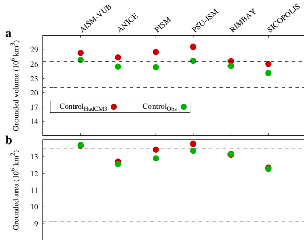
Fig. 4. a) Final grounded ice volume ( 10^6 \text{ km}^3 ) and b) final grounded ice area ( 10^6 \text{ km}^2 ) for the control simulations with Bedmap1. \text{Control}_{\text{HadCM3}} in red, \text{Control}_{\text{Obs}} in green. The horizontal dashed lines indicate the PD and Pliocene grounded ice volume and area of the initial ice-sheet topographies.
