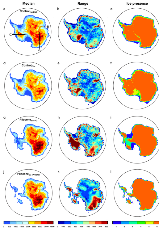
Fig. 9. Median, range and coverages of grounded and floating ice thickness from the six ISM simulations with Bedmap1. From top to bottom shows the main four experiments. All six ice thickness values for all locations are sorted, the median is shown as the mean of the 3th and 4th value (in m), the range is the difference between the 6th and the 1st, divided by two and ice coverage counts if any ice is present (0: no ice, 6: all ISMs have ice). The black lines in panel a) represent the cross sections shown in Fig. 10: A - Wilkes basin, B - Lambert ice stream and C - the WAIS.
