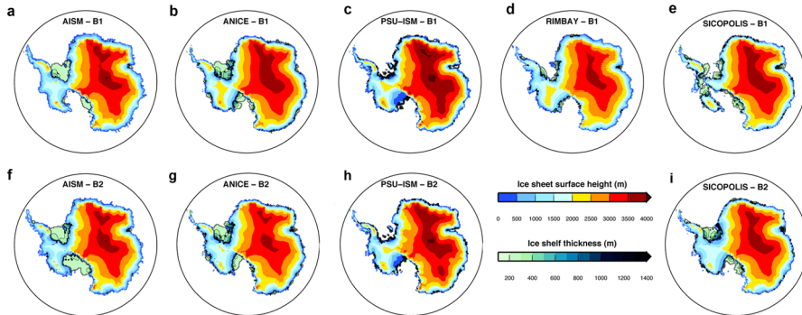
Fig. 8. Ice surface topography and ice thickness of the ice shelves for the Pliocene PD-Ant simulations with HadAM3 Pliocene climate forcing except a modern Antarctica. All models are initialised with their own Control HadCM3 final ice-sheet (Fig. 3). Panels a-e show simulations with Bedmap1, panels f-i show simulations with Bedmap2. For all panels the colour scale is the same as in Fig. 3. a,f) AISM-VUB, b,g) ANICE, c,h) PSU-ISM, d) RIMBAY, e,i) SICOPOLIS.
