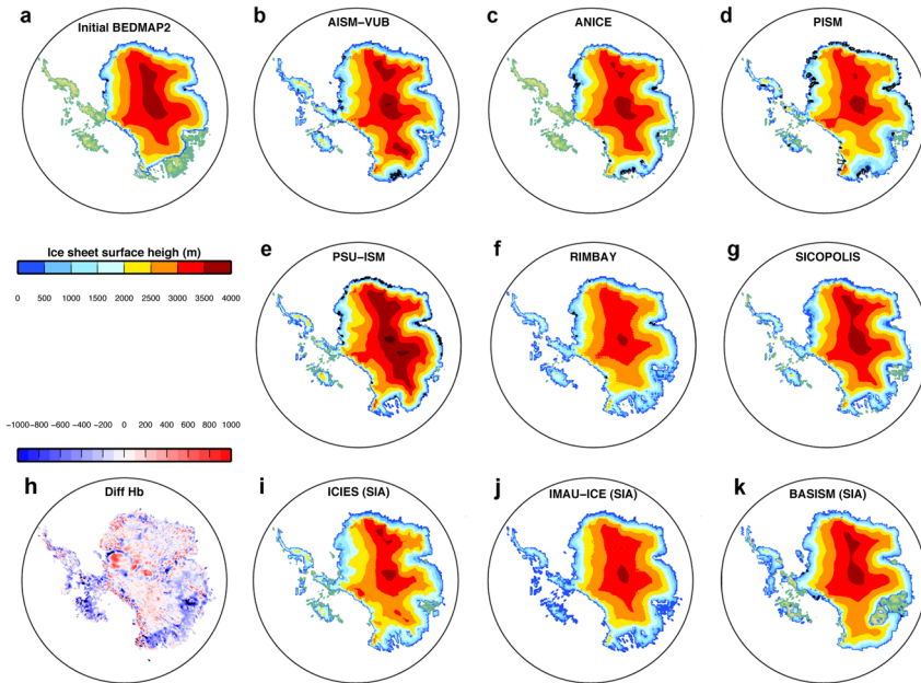
Fig. 11. Ice surface topography and ice thickness of the ice shelves for the Pliocene Ice-PRISM3 simulation with Bedmap2. a) The initial PRISM3 ice sheet topography modified for Bedmap2 (see text for details). b) AISM, c) ANICE, d) PISM, e) PSU-ISM, f) RIMBAY, g) SICOPOLIS. h) Difference between Bedmap2 and Bedmap1 bedrock topography for the PRISM3 initial ice sheet. SIA-only models; i) ICIES, j) IMAU-ICE, k) BASISM.
