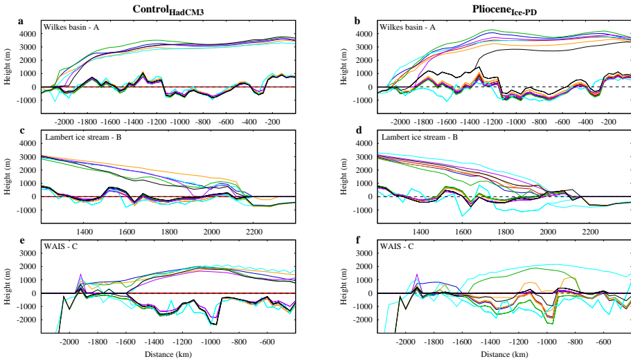
Fig. 10. Cross section through the ice sheets showing surface and bedrock topographies. Cross sections as indicated in Fig. 9. Top row shows a cross section of the Wilkes basin (A), middle panels show the Lambert ice stream (B) and bottom panels a cross section through the West Antarctic ice sheet (C). Left panels show the \text{Control}_{\text{HadCM3}} simulation, the right panels for the \text{Pliocene}_{\text{Ice-PD}} simulations. The colours represent the different models and match with the lines in Fig. 2, black lines indicate the PD topography (panels a,c,e) and the PRISM3 topography (panels b,d,f) of Bedmap1.
