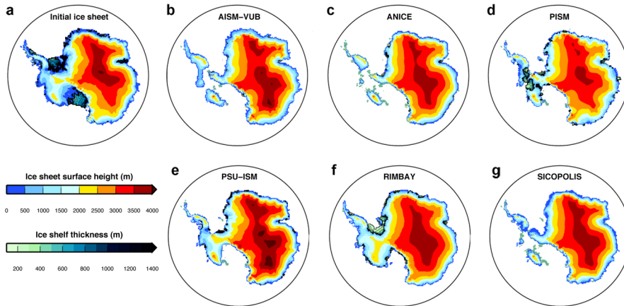
Fig. 5. Ice surface topography and thickness of the ice shelves for the Pliocene Ice-PD simulation, with HadCM3 Pliocene climate forcing. a) Initial ice sheet from Bedmap1, b) AISM, c) ANICE, d) PISM, e) PSU-ISM, f) RIMBAY, g) SICOPOLIS.
