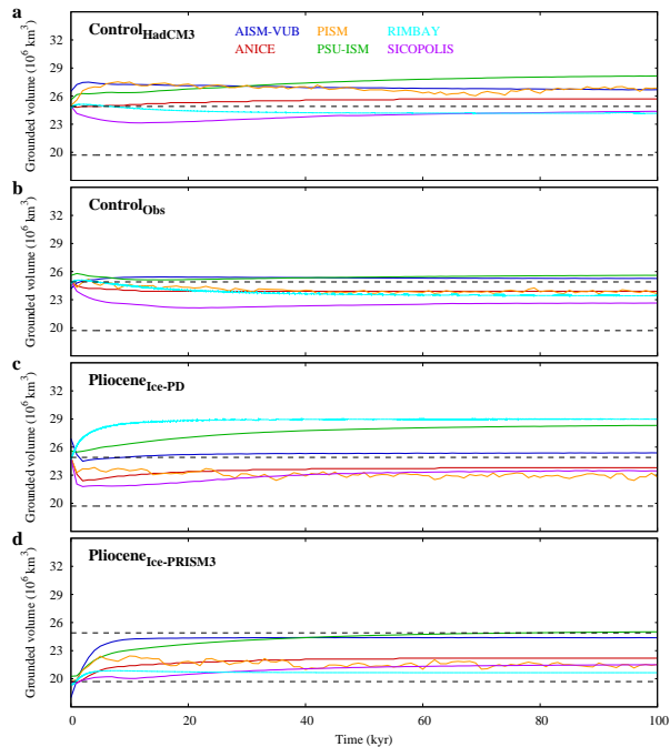
Fig. 2. Modelled grounded ice volume over 100 kyr with Bedmap1. a) The \text{Control}_{\text{HadCM3}} simulation, with HadCM3 pre-industrial climate forcing. b) The \text{Control}_{\text{Obs}} simulation, with ERA-40/WOD09 climate forcing. c) The \text{Pliocene}_{\text{Ice-PD}} simulation, with HadCM3 Pliocene climate forcing and an initial PD ice sheet. d) The \text{Pliocene}_{\text{Ice-PRISM3}} simulation, with HadCM3 Pliocene climate forcing and the initial PRISM3 ice sheet. The horizontal dashed lines indicate the PD and Pliocene grounded ice volume of the Bedmap1 ice-sheet topographies.
