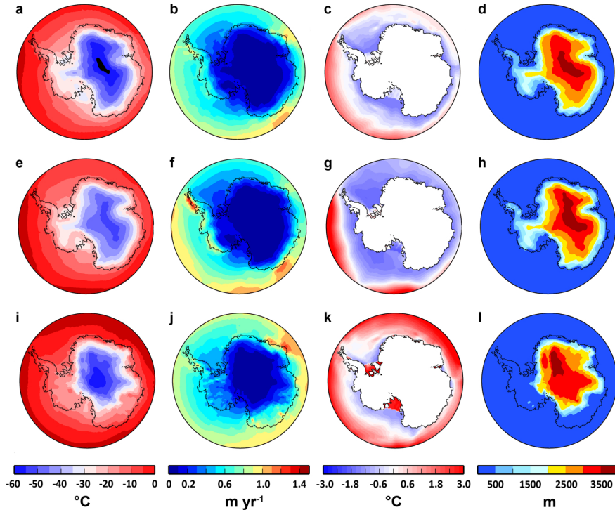
Fig. 1. Yearly mean climatology of the three different climate forcing used (see Table 1). Top panels shows results from a pre-industrial run of HadCM3. Middle panels is ERA-40 (1971-2000 reanalysis) (Uppala et al., 2005) and ocean temperatures from the WOD-09 data set (Boyer et al., 2009). Bottom panels illustrate the Pliocene HadCM3 run with full PRISM3 boundary conditions (Haywood et al., 2011). From left to right, surface-air temperature in ^{\circ}\text{C} , Precipitation in \text{m yr}^{-1} water equivalent, sea surface temperatures and temperatures at the bottom of the PD ice shelves in ^{\circ}\text{C} and surface topography in the climate model in m. The black line in all panels represents the Bedmap1 outline of the grounding line.
