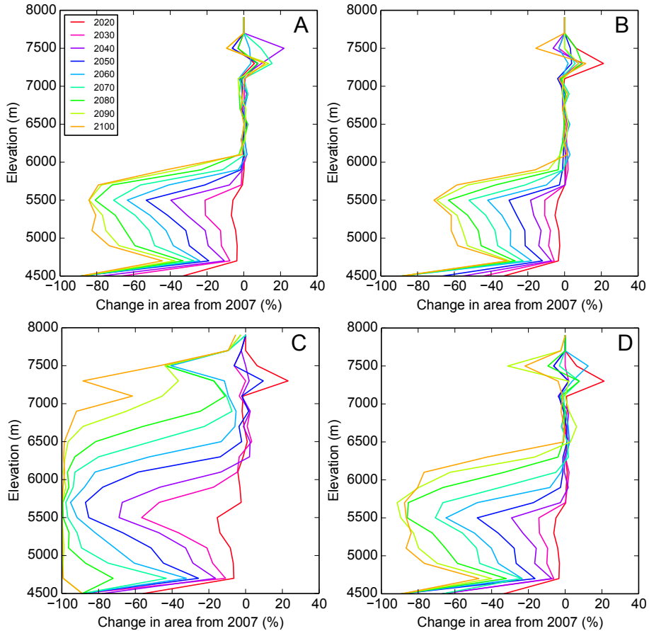
Figure 17. Change in glacier area versus elevation for (A) the dry/warm RCP4.5 scenario, (B) the wet/cool RCP4.5 scenario, (C) the dry/warm RCP8.5 scenario, and (D) the wet/cool RCP8.5 scenario.
