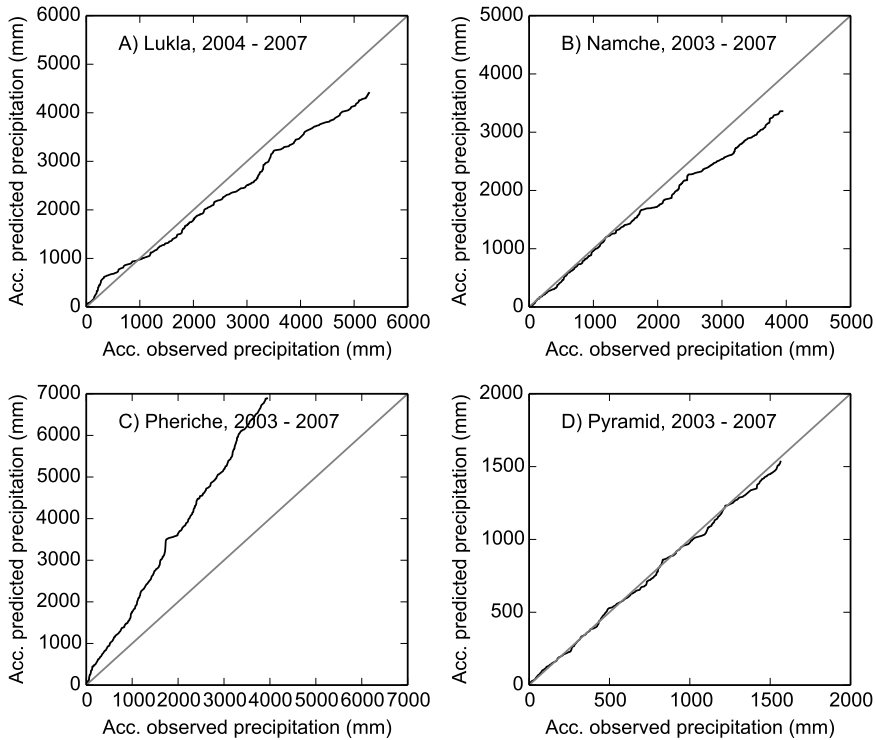
Figure 6. Accumulated observed and predicted precipitation at the EVK2CNR sites. Days where T < 0 or precipitation observations were missing were excluded from the analyses.
