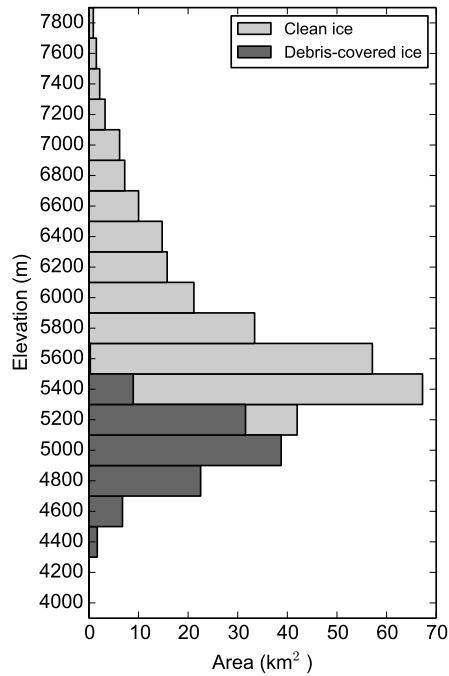
Figure 2. Area of clean and debris-covered glaciers by elevation, Dudh Kosi basin, Nepal. Extracted from SRTM 90 m DEM and glacier inventory from ICIMOD (2011)
