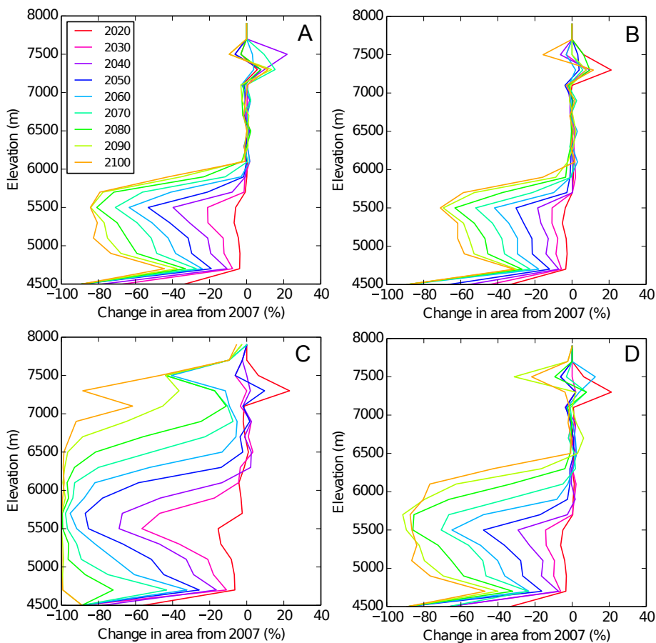
Figure 16. Change in glacier area versus elevation for (A) the dry/warm RCP4.5 scenario, (B) the wet/cool RCP4.5 scenario, (C) the dry/warm RCP8.5 scenario, and (D) the wet/cool RCP8.5 scenario.
