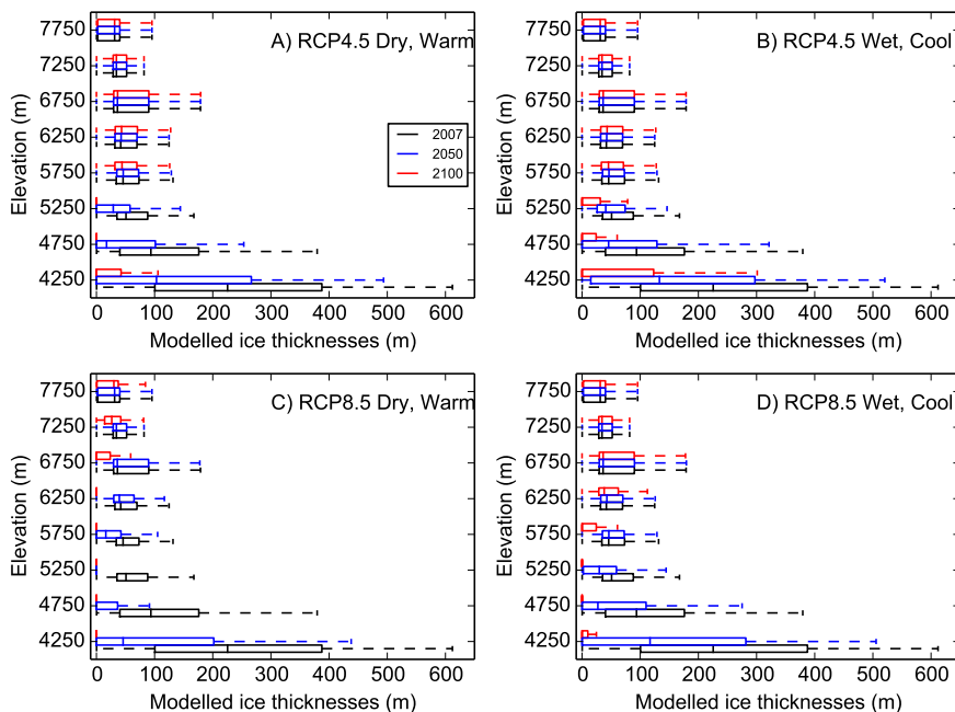
Figure 17. Distribution of modeled ice thicknesses by elevation band, for 2007 (initialization), 2050, and 2100. (A) dry/warm RCMP4.5 scenario, (B) wet/cool RCP4.5 scenario, (C) dry/warm RCP8.5 scenario, and (D) wet/cool RCP8.5 scenario.
