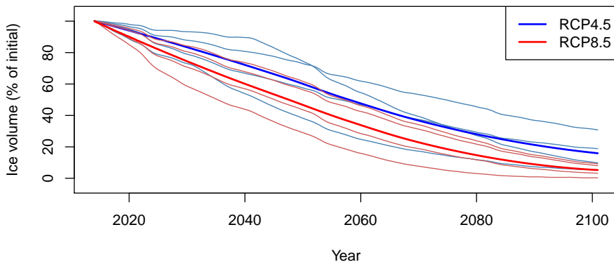
Figure 15. Sensitivity of modelled glacier volumes to decadal T and P anomalies from four RCP4.5 (blue) and four RCP8.5 (red) ensemble members (see Table 5 for details. Realizations are given as thin lines, and ensemble means are thick lines. All realizations are smoothed with a loess filter (span = 0.05) to minimize interannual variations.
