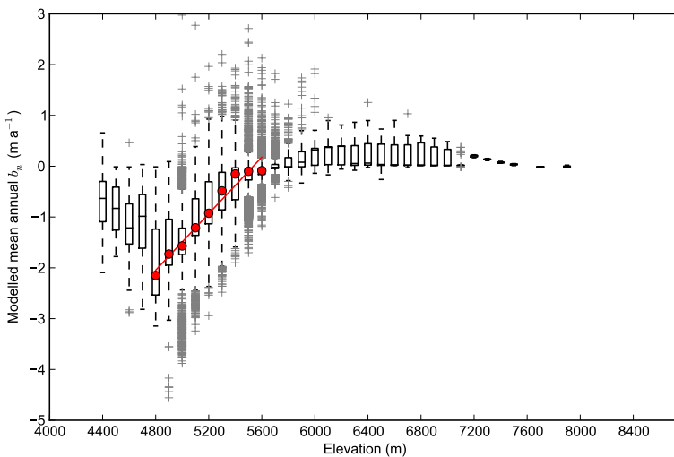
Figure 12. Boxplots of modelled mean annual mass balance ( \text{m w.e. yr}^{-1} ) calculated for 100 m intervals (1961 - 2007). Calculated mass balance gradient of 0.27 \text{ m (100 m)}^{-1} between 4850 and 5650 m is shown in red.
