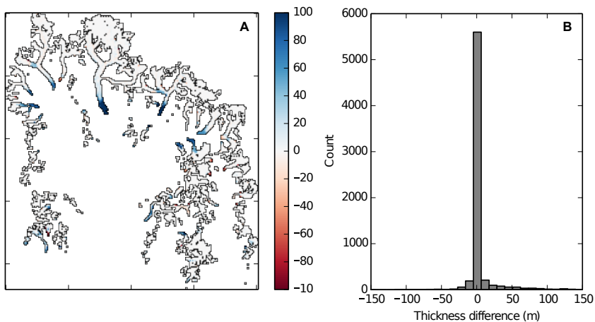
Figure 8. A) Differences in modeled ice thickness (in m) between the end of the first initialization run (47 years), and after an additional 94 years of simulation with dT = -1.2C . B) Histogram of differences in modeled ice thickness.
