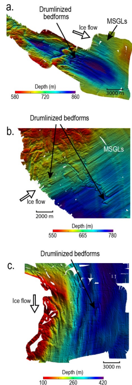
Figure 3. Close-up on the seabed morphology and swath bathymetry perspective views. The location of (a)–(c) is presented in Fig. 2. Offshore topography is gridded at 25 m and showed with a vertical exaggeration of X3 (a) Bathymetry image showing the Cold Seep Basin region with drumlinized bedforms and Mega Scale Glacial Lineations (MSGLs) associated to a paleo-ice flow direction, (b) SCAR Inlet, and (c) Cape Framnes, south of the Jason Peninsula. The paleo-ice flow direction is indicated by the white narrow.
