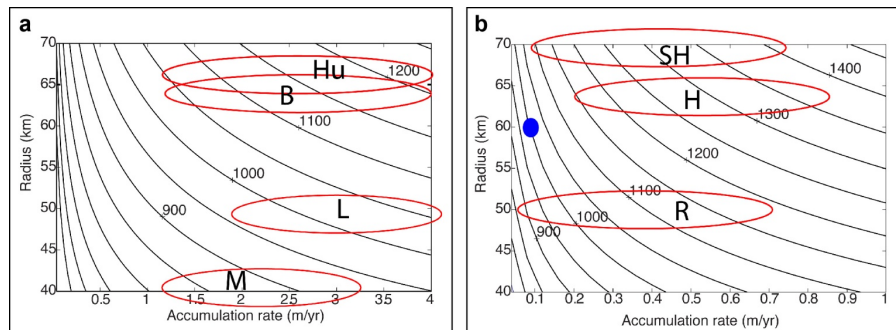
Figure 8. Range of ice thickness expected from (a) Marr (M), Livingston (L), Brabant (B), and Hugo (Hu) west AP continental-shelf domes where the ice temperature is assumed to average 0^{\circ}\text{C} , and (b) Robertson (R), Hektoria (H), and Snow Hill (SH) east AP continental-shelf domes with ice averaging -10^{\circ}\text{C} using the Bodvarsson–Vialov model (Bueler et al., 2005). The blue dot is the modern analog Siple Dome in West Antarctica of 1000 m thick that fits well the model. See Fig. 5 for the location of the domes.
