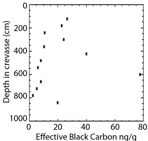
Figure 9. eBC from snow samples collected from the walls of a crevasse on Vallunaraju (region 4) the nearest high mountain to Huaraz. A decreasing trend with depth is noted. These lowest samples were visually the cleanest snow samples from the crevasse walls, and were likely to have accumulated during the wet season. The points at 400, 600, and 850 cm were thin noticeably dark layers.
