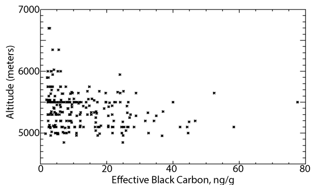
Figure 6. Complete dataset of eBC values determined from the LAHM analysis plotted vs. altitude.
