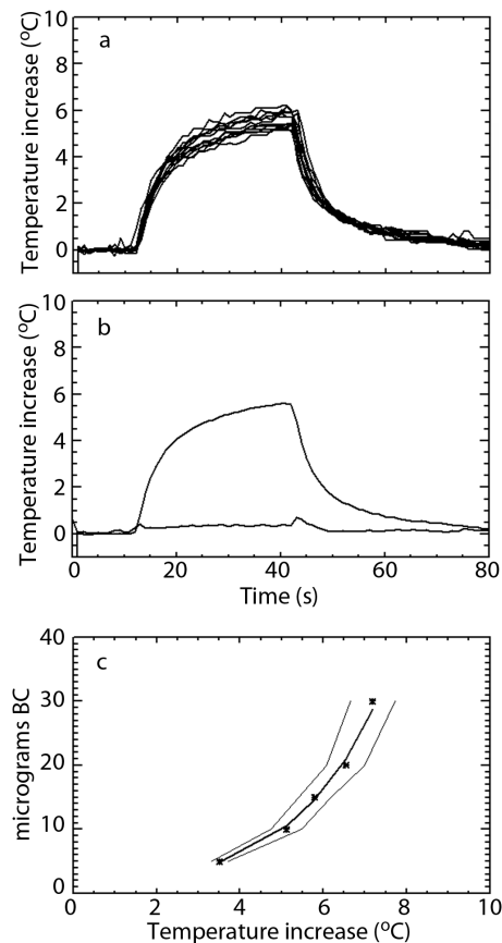
Figure 3. (a) Twelve temperature profiles measured for filters with 10 micrograms of fullerene soot. Profiles are from three different filters measured four times each. (b) Mean temperature profile and SD of data 12 temperature profiles. (c) Temperature increases after ten seconds for five masses of fullerene soot. Error bars are SDs for each measurement and bold line is fit to data.
