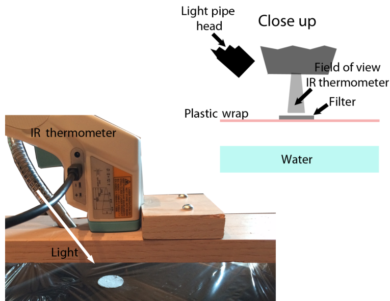
Figure 1. Diagram of the LAHM analysis setup. A light source is aimed at a 45^\circ angle at the filter which rests on plastic wrap approximately 10 cm above the water surface. The IR thermometer directly views the center of the filter. The field of view of the thermometer is approximately 1.5 cm at the distance of the filter and the contaminant spot on the filter is generally 2 cm in diameter.
