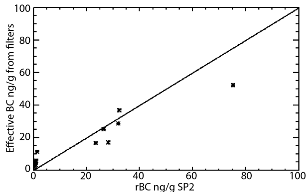
Figure 5. Plot showing the relationship between eBC as determined from the LAHM analysis and refractory black carbon as determined by the SP2 instrument ( r^2 = 0.92 ). The values near 0.0 rBC are from Pisco mountain in region 2 while the higher values are from Vallunaraju in region 4. The 1 to 1 line is plotted to guide the eye.
