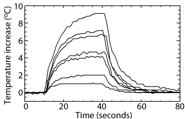
Figure 2. Measured temperature profiles for 7 filters with a variety of light absorbing particulate loads. Temperature recording started ten seconds before the lamp was illuminated, and the lamp was extinguished 30 s later. Temperatures are normalized to the average of first 10 s of data and the temperature usually returned to the start temperature within a minute of the lamp being extinguished.
