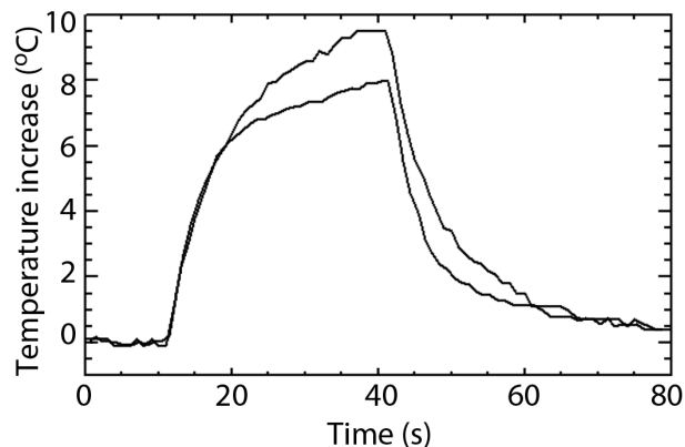
Figure 4. Temperature profiles measured for a calibration filter with fullerene soot (lower curve), and a sample filter with dust and black carbon (upper curve). The curves are nearly identical until 20 s (10 s of heating) after which they diverge. The continued more rapid increase in temperature of the dust–black carbon mixture is thought to be due to the dust.
