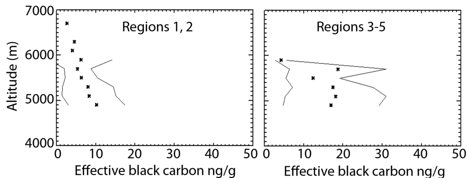
Figure 8. LAHM determined eBC values averaged by altitude bins plotted with \pm 1 SD (lines) by altitude for the northern (regions 1 and 2) mountains and the southern (regions 3–5) mountains in the Cordillera Blanca. Absorbing particulates in snow in regions 1 and 2 are likely primarily dust while regions 3–5 are strongly influenced by pollution from the city of Huaraz.
