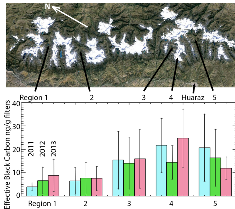
Figure 7. Google map image of the Cordillera Blanca mountain range. The five regions as well as the city of Huaraz are indicated on the map by black arrows. Average eBC values as determined from the LAHM analysis are shown in the plot for each of the three years. The thin lines indicate \pm 1 SD of the measurements. Note that in 2013, region 2, SP2 samples averaged 0.65 \text{ ng g}^{-1} rBC indicating that most of the 5 \text{ ng g}^{-1} of the eBC estimate could be due to light absorption by dust.
