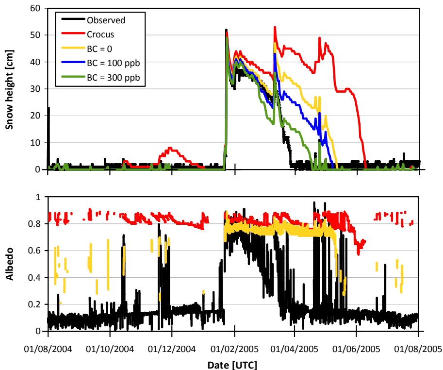
Figure 3. Top panel: comparison of observed (black) and simulated snowpack heights at NCO-P for the winter season 2004/05. Simulations were performed with the standard crocus model (red) and with the upgraded model including radiative transfer with constant BC concentrations of 0 (yellow), 100 (blue), and 300 ppb (green). Snowpack heights simulated with the upgraded model are indistinguishable for the different BC concentrations until late January and after mid-May. Bottom panel: comparison of observed (black) and simulated albedo at NCO-P. Simulations were performed with the standard crocus model (red) and with the upgraded model including radiative transfer but without BC (yellow).
