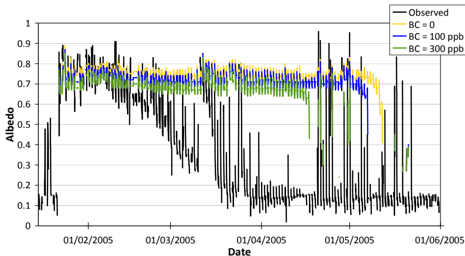
Figure 5. Comparison of observed (black) and simulated albedo at NCO-P for the period 15 January to 1 June 2005. Model results are obtained with the upgraded model including radiative transfer with different BC concentrations: 0 (yellow), 100 ppb (blue), and 300 ppb (green).
