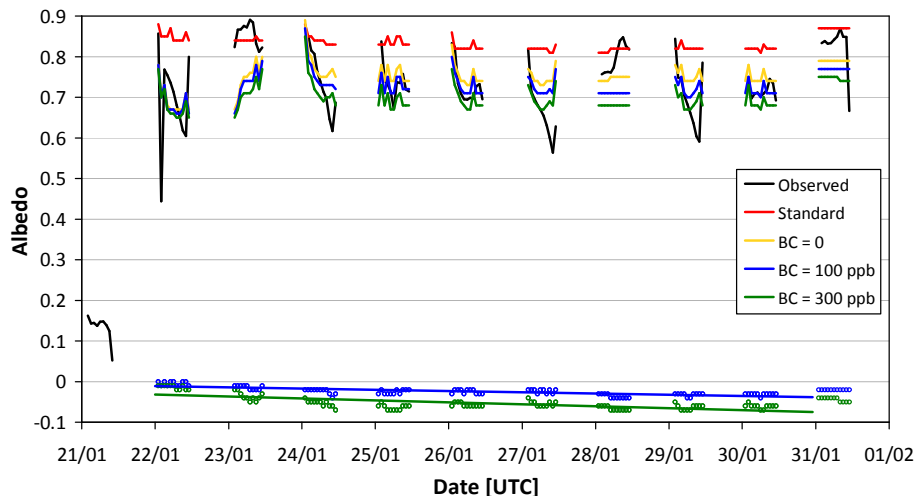
Figure 4. Comparison of observed (black) and simulated albedo at NCO-P for the period 22 to 31 January 2005. Model results are obtained with the upgraded model including radiative transfer with different BC concentrations: 0 (yellow), 100 ppb (blue), and 300 ppb (green). Circles at the bottom indicate the differences of the simulated albedo between BC = 100 ppb and 0 (blue) and BC = 300 ppb and 0 (green). Straight blue and green lines show the results obtained by linear regressions for the albedo differences during the period 22 to 30 January 2005.
