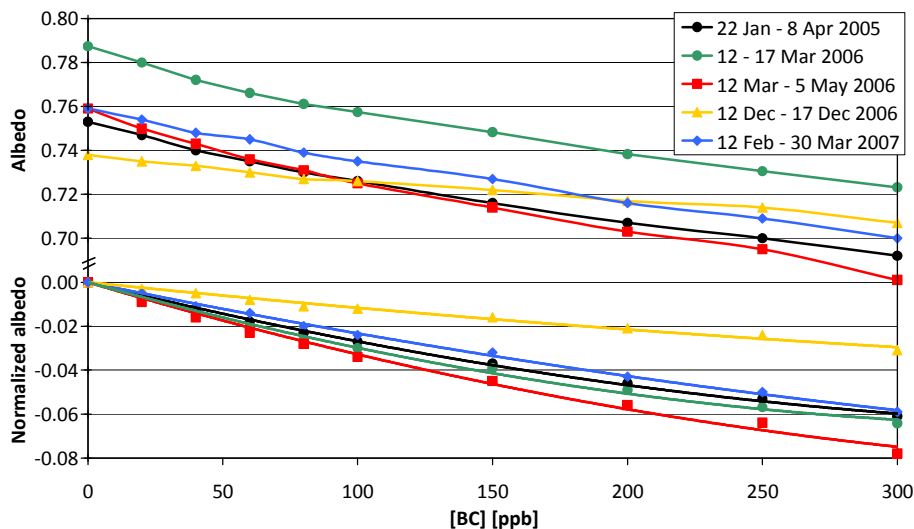
Figure 6. Top panel: simulated average albedo for several periods with continuous snow higher than 10 cm as a function of BC concentration. Bottom panel: normalized albedo as differences of the averaged albedo minus the averaged albedo at BC = 0. The lines correspond to the best fit of a quadratic polynomial forced through zero for each set of the normalized albedo.
