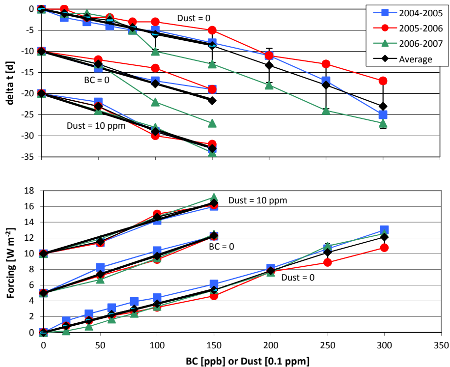
Figure 7. Top panel: reduction in the snow-covered period in days simulated for different BC and dust concentrations in the snow. Bottom panel: simulated annual radiative forcing related to shortwave radiation due to the presence of BC and dust in the snow. Simulations are performed without dust, without BC (shifted by -10 days or +5 \text{ W m}^{-2} ), and with dust = 10 ppm (shifted by -20 days or +10 \text{ W m}^{-2} ). In the last case, the reductions are calculated relative to the case with BC = 0 and dust = 10 ppm. Black symbols indicate the 3 year averages of the radiative forcing with the error bars representing the SD. Black lines correspond to linear regressions forced through the origin for the average values for BC \leq 150 ppb.
