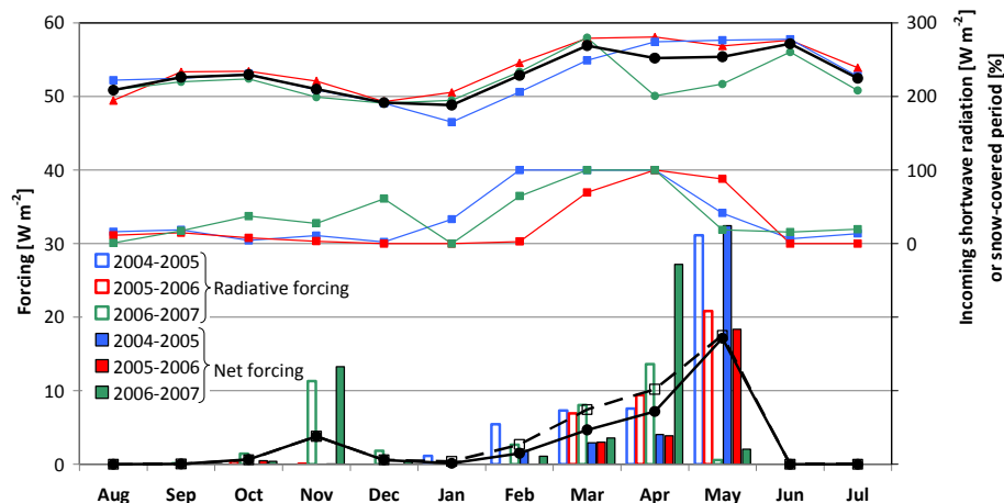
Figure 8. Simulated monthly mean radiative (open bars) and net forcing (filled bars) for the seasons 2004/2005 (blue), 2005/2006 (red), and 2006/2007 (green) due to the presence of 100 ppb of BC in the snow. Black open squares and filled circles indicate 3 year averages of the monthly means of the radiative and net forcing. Also shown are snow-covered periods in percent based on the simulations without BC in the snow (middle) and the monthly means of the observed incoming short-wave radiation (top) for the three years. The black circles in the top panel indicate the 3 year average of the monthly means of the incoming radiation.
