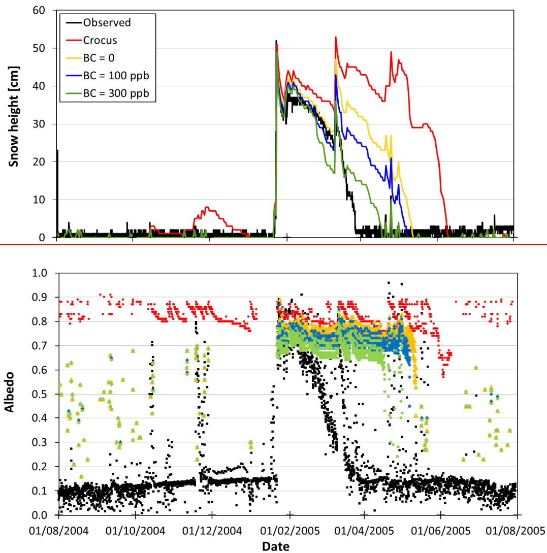
Figure 3. Comparison of observed (black) and simulated snowpack heights (top) and albedo (bottom) at NCO-P for the winter season 2004/05. Simulations were performed with the standard crocus model (red) and with the upgraded model including radiative transfer with constant BC concentrations of 0 (yellow), 100 (blue), and 300 ppb (green). Snowpack heights simulated with the upgraded model are indistinguishable for the different BC concentrations until late January and after mid-May.
