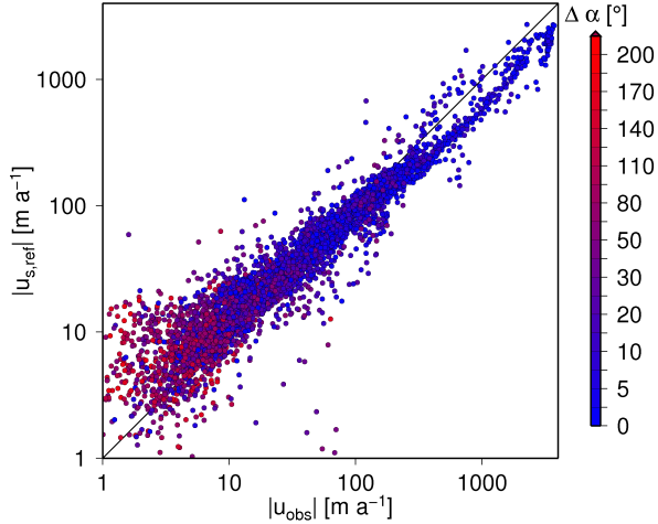
Figure 5. Observed surface velocity field |u_{\text{obs}}| vs. reference surface velocity field |u_{\text{s,ref}}| . The logarithmic scales exaggerate the spread around the low speeds. The angle offset \Delta\alpha between the vectors of the surface velocity field u_{\text{obs}} and the reference surface velocity field u_{\text{s,ref}} is shown as the colour code.
