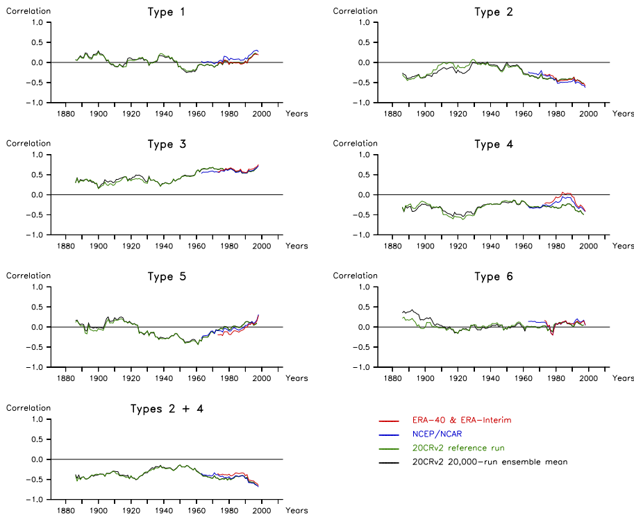
Figure 4. The 30 year running correlation is calculated between the annual (JJA) SLP-based frequencies of each type and the JJA CRU NAO index. For the “Types 2 + 4” correlation, the frequencies of Types 2 and 4 have been summed before computing the correlation.
