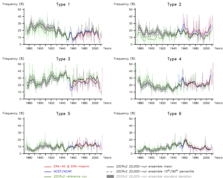
Figure 2. The solid lines are calculated as the 10 year binomial running mean frequencies and the dotted light lines are the corresponding annual (JJA) SLP-based frequencies.
