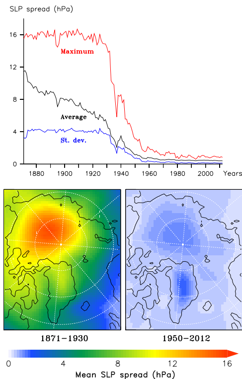
Figure 3. Top: the average SLP spread and its standard deviation are calculated as the seasonal (JJA) average 20CRv2 spread and its standard deviation over the oceanic pixels of our domain. The maximum SLP spread is the value of the oceanic pixel showing the highest seasonal (JJA) average spread of each year. Bottom: the SLP spread is calculated as the average 20CRv2 spread over the 1871–1930 summers (JJA), left, and over the 1950–2012 summers, right.
