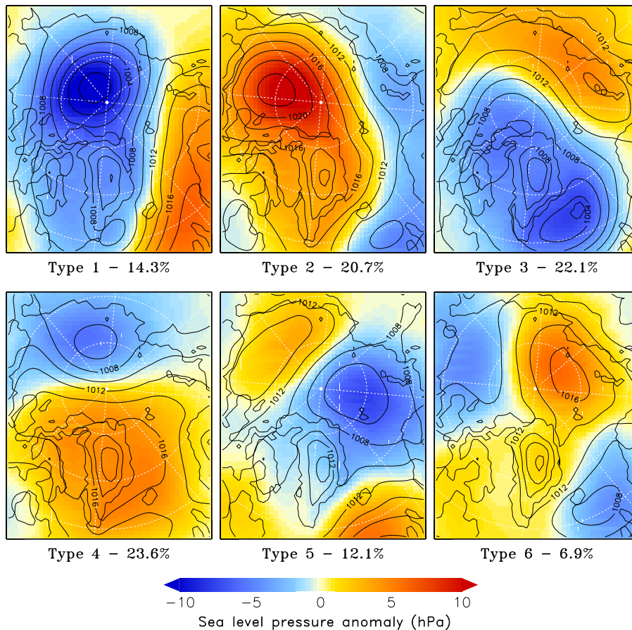
Figure 1. The SLP-based reference circulation types over the 1980–2012 (JJA) period for ERA-Interim are represented by the solid black isobars (in hPa). The SLP anomaly (in colours) is calculated as the difference between the class mean SLP and the seasonal mean SLP over 1980–2012. The average frequency of each type is also given.
