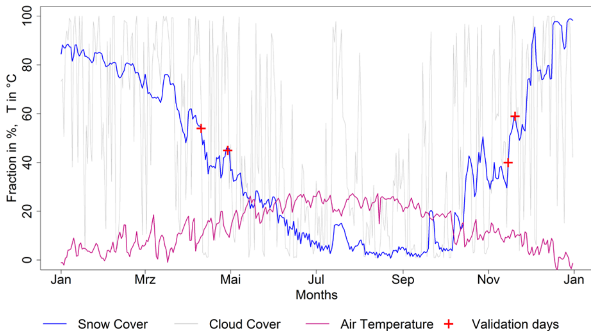
Figure 1. Snow cover area dynamics in the Zerafshan basin derived from MODIS daily snow cover time series for the year 2004. Cloud removal from original MODIS snow cover product is done using the methodology by Gafurov and Bárdossy (2009). Air temperature is from Pendjikent meteorological station (see Figure 1 in the submitted manuscript).
