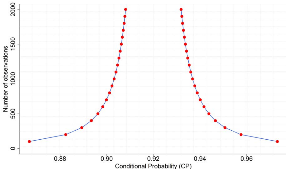
Figure 3. Confidence interval (95 %) derived from binomial distribution against number of observations, exemplarily plotted for P(S_p|S_s)=0.92 .
