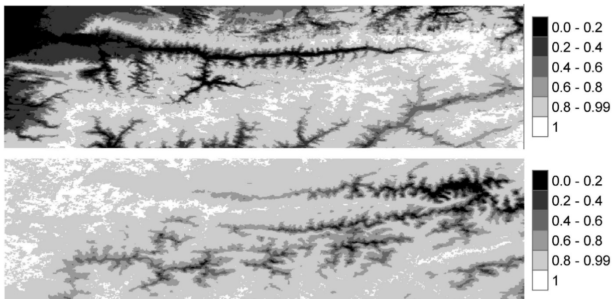
Figure 4. MR^S (top) and MR^l (bottom) maps of the Chimgan station (see Fig. 1) for the study area. The figure shows the same domain as Figure 1b
