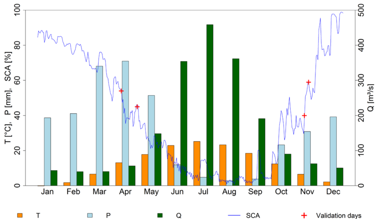
Figure 2. Monthly average air temperature (T), cumulative precipitation (P), discharge (Q) and SCA dynamics in the Zerafshan basin. T, P and Q means are based on data for the period from 1930 till 2008. Daily SCA is for 2004 obtained from MODIS and cloud eliminated using Gafurov and Bárdossy (2009). Temperature (zero in January) and precipitation data are from the Pendjikent station (1016 m a.s.l.), discharge is measured at the Dupuli gauge (see Fig. 1).
