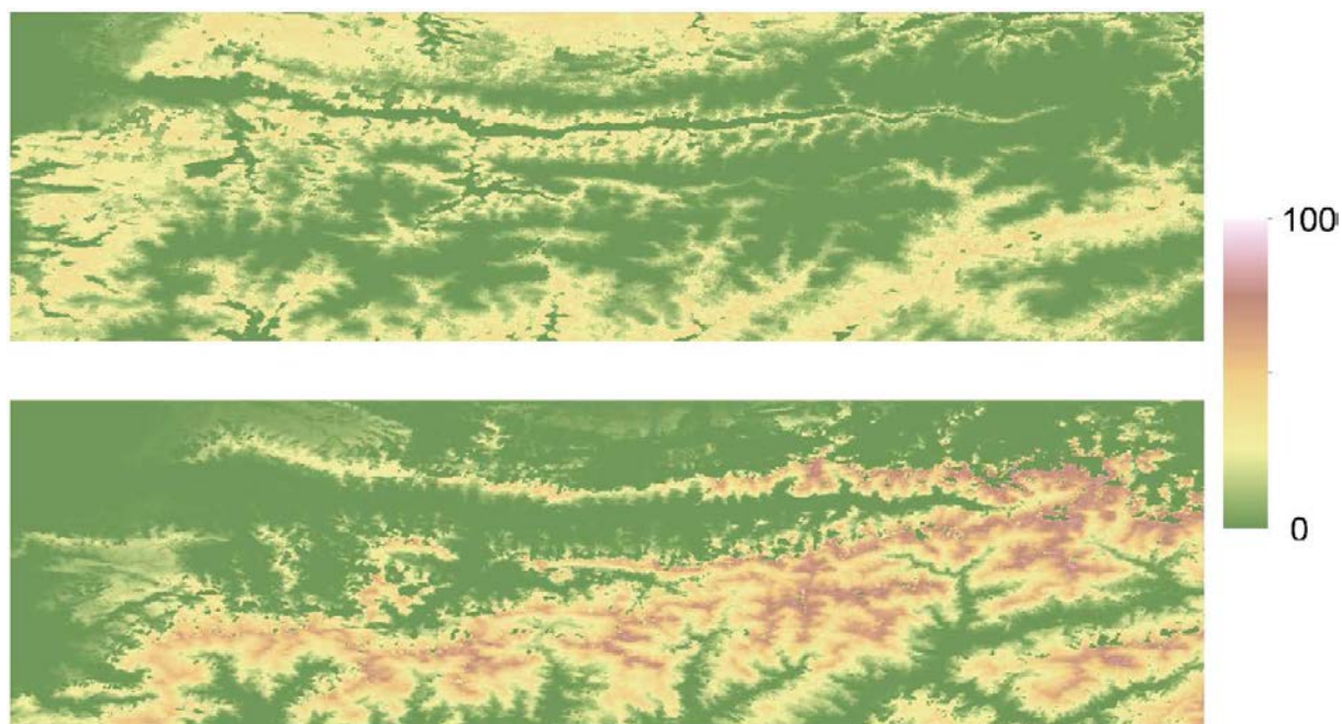
Figure 7. SPI (top) and LPI (bottom) values of each pixel (in %) in the study area defined in Fig. 1b.
