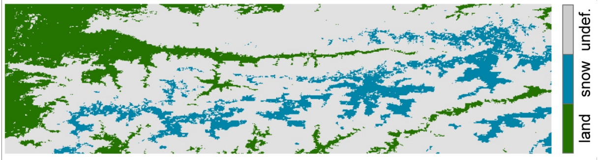
Figure 5. Temporally persistent spatial snow ( MP^S = 1 ) and land ( MP^L = 1 ) patterns for April in the study area shown in Fig. 1b. Pixels with “undef” indicate MP^S < 1 or MP^L < 1 , for which classification is not possible in this step.
