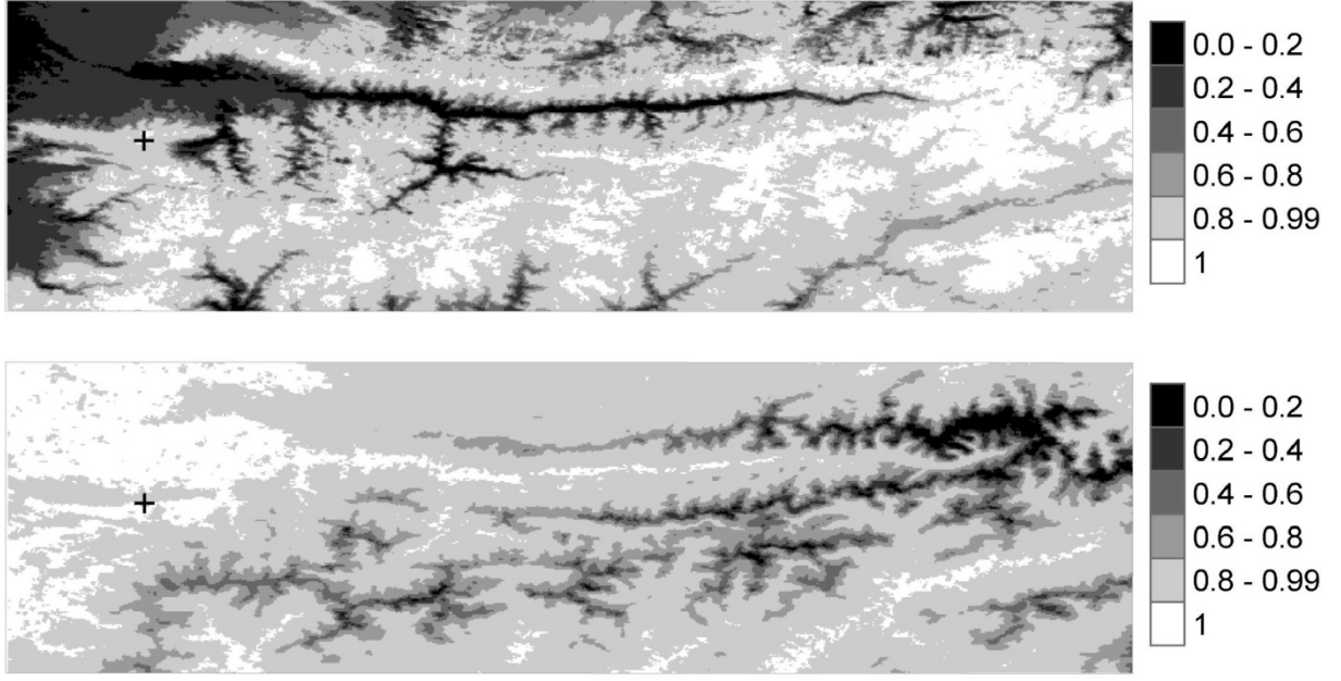
Figure 6. MR^s_{(i,j),(100,100)} (top) and MR^l_{(i,j),(100,100)} (bottom) fields for the pixel x = 100 , y = 100 (black cross) with elevation 2206 m.a.s.l.
