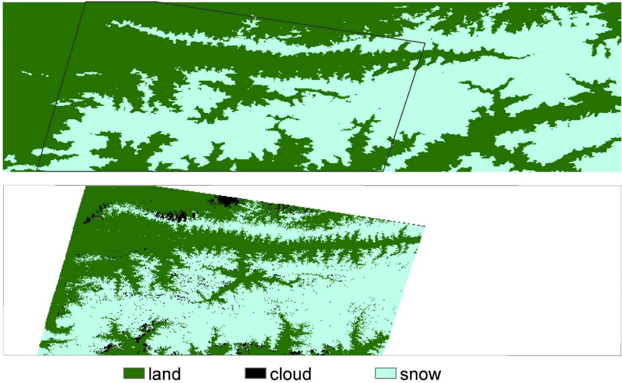
2 Figure 8. Reconstructed (top) and Landsat (bottom) snow cover maps for April 10, 1998.
