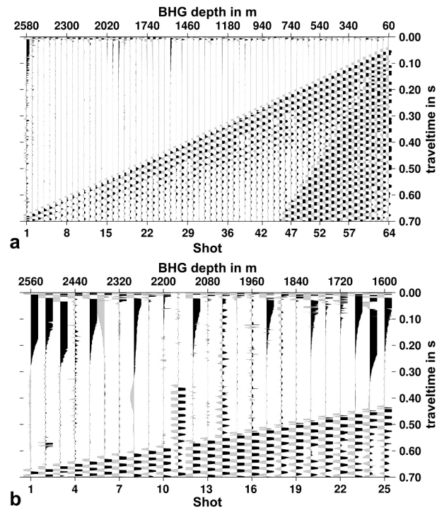
Figure 4. Recorded first arrivals from the VSP surveys with detonation cord ( a , survey 20130545) and booster ( b , survey 20130546) as source. The top ordinate gives the location, hence, the depth of the borehole geophone (BHG), the bottom ordinate shows the shot number. In ( a ) not only the direct P-wave arrival is visible but also a borehole guided wave travelling with a velocity of 1150 \text{ m s}^{-1} . Depth is given here to top of casing.
