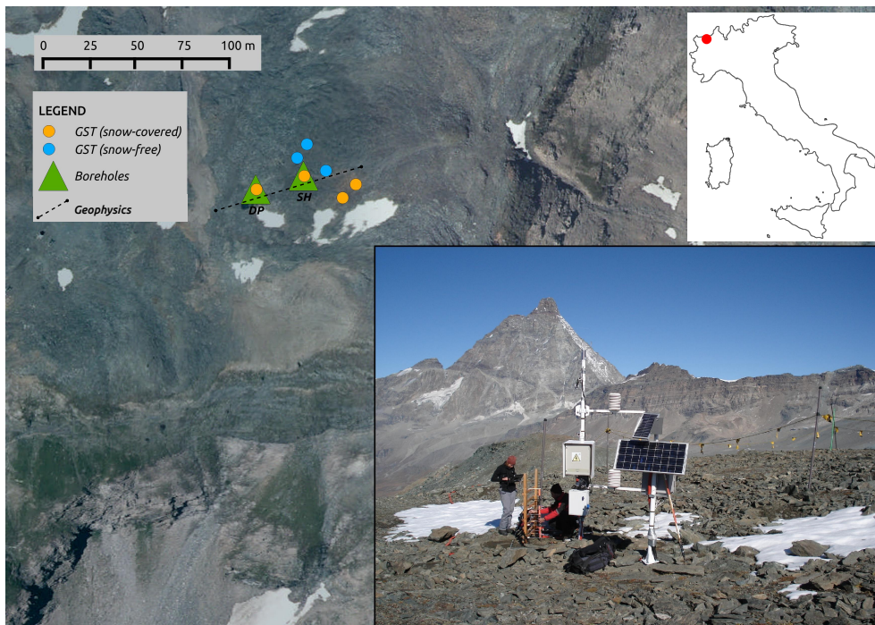
Figure 1. Overview of the Cime Bianche monitoring site.
