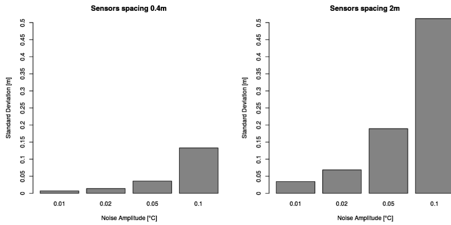
Figure 5: Uncertainty of ALT estimation as function of noise amplitude. Left: for sensor spacing of 0.4m (case of SH). Right: for sensor spacing of 2 m (case of DP).
