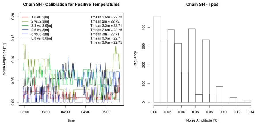
Figure 2: Calibration experiment of chain SH, positive temperatures. Top: temperature variations vs. time. Bottom left: noise amplitude of each pair vs. time. Bottom right: frequency distribution of the noise amplitudes of all pairs.
