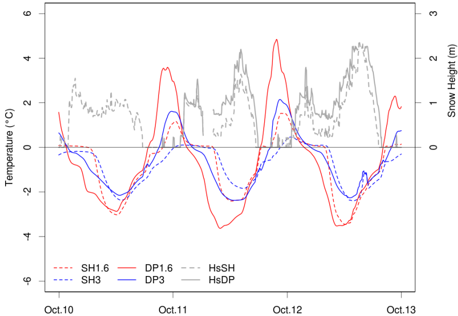
Figure 6. Fluctuations of snow cover thickness (Hs) and ground temperatures (daily mean) at selected depths in the active layers of Cime Bianche from 1 October 2010 to 30 September 2013-2013 determined from borehole temperature data . Lines type: dashed is for SH, solid is for DP. Colors: red is for shallower temperatures (1.6 m), blu is for deeper temperature (3 m), grey is for snow.
