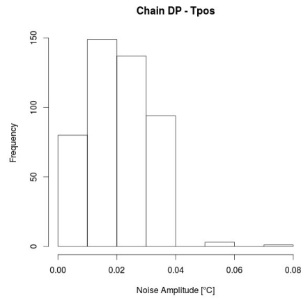
Figure 4: Calibration experiment of chain DP, positive temperatures. Top: temperature variations vs. time. Bottom left: noise amplitude of each pair vs. time. Bottom right: frequency distribution of the noise amplitudes of all pairs.
