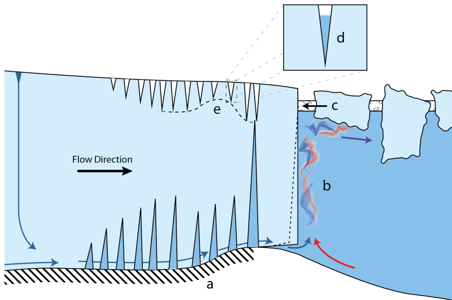
Figure 4. Proximal and distal processes affecting calving. (a) Varying basal friction ( \tau_b ) affects the stress field in the glacier. (b) Changing fjord water temperatures and, more importantly, subglacial water flux affect the rate of submarine melting of the calving face and floating tongue (when present). (c) The seasonal formation of mélangé provides a buttressing force which suppresses surface crevasse depth and, thus, calving. (d) Surface melt water in crevasses causes hydrofracturing, which acts to deepen surface crevasses. (e) Glacier geometry exerts a strong influence on crevasse field depth. Compressional forces on the stoss side of Store's pinning point suppress the depth of crevasses, while rapid loss of basal traction in the lee side deepen them.
