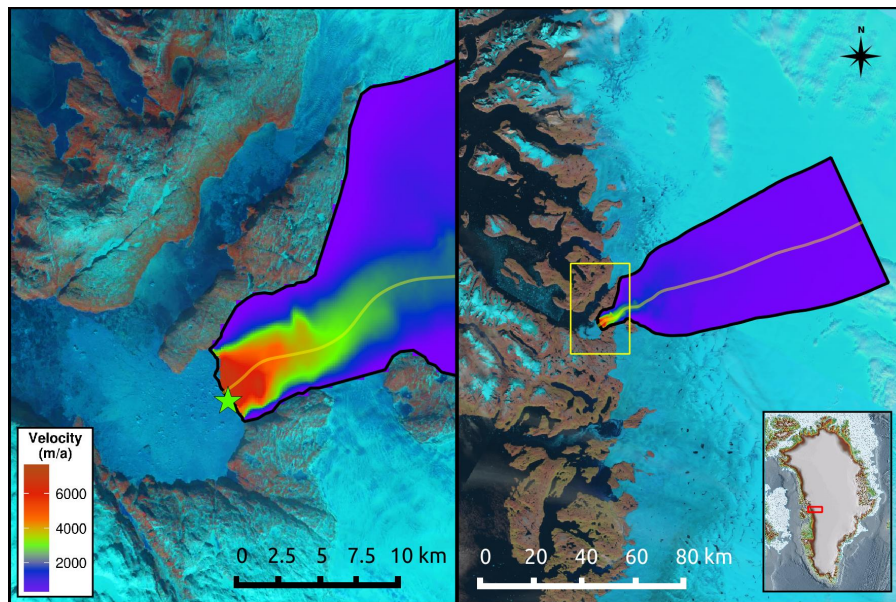
Figure 1. Store Gletscher in Ikerasak Fjord, Greenland. Colour scale shows summer velocity ( \text{m a}^{-1} ) from the MEaSUREs program (Joughin et al., 2011). Yellow line indicates the flowline used in this study, and the green star indicates the location of the main proglacial plume forming where subglacial water is discharged into the fjord.
