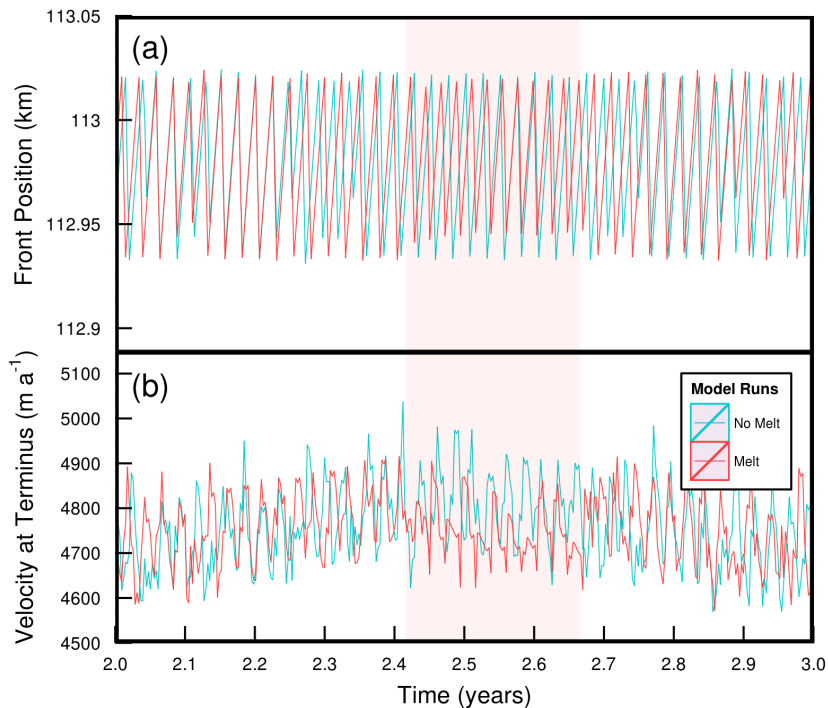
Figure 5. Plots showing variations in terminus position (a) and velocity (b) , over the course of a year for baseline model run (blue line) and run with submarine melting applied (red line). Red shading indicates melt season. The saw-toothed pattern in both panels is a result of calving.
