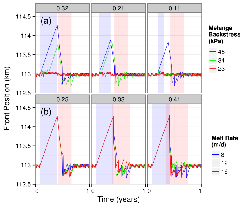
Figure 9. Plots showing terminus position through one year for varying mélange season length (a) and melt season length (b) . Durations of mélange and melt season are indicated by blue and red shading (and panel title), respectively, varying from left to right, with colour indicating the magnitude of the perturbation. Moving from left to right panels, and moving from blue, through green, to red line colours, indicate progressively more severe “warming climate” scenarios.
