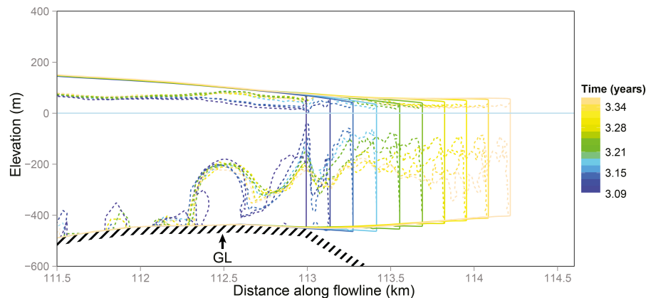
Figure 7. Sequential profiles of Store Gletscher during advance of its calving terminus due to mélange backstress. As the floating tongue advances from the grounding line (marked GL), it rises upwards due to buoyant forces, which also act to close surface crevasses near the grounding line. This indicates that flow dynamics at the grounding line are forcing the terminus below flotation.
