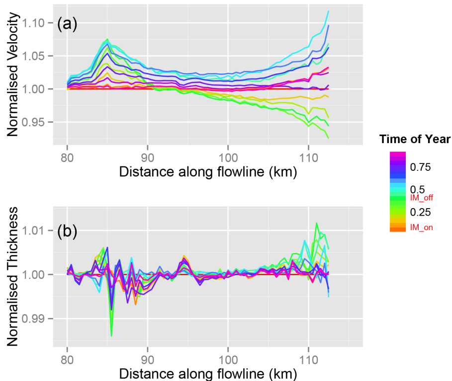
Figure 8. Plots showing velocity (a) and thickness (b) perturbations through a single year. Line colour indicates time of year. Velocity and thickness have been normalised against their Jan 1 values.
