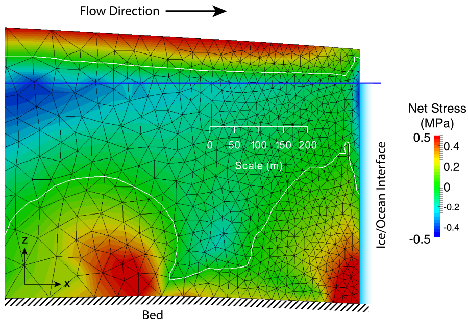
Figure 3. The terminus of the flowline mesh of Store Gletscher. White line indicates the net stress ( \sigma_n ) zero contour for both surface and basal crevasses. Blue line indicates sea level. Net stress (MPa) is > 0 where crevasses exist and < 0 in solid and unfractured ice. Calving occurs in the model when surface and basal crevasses meet.
