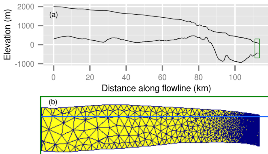
Figure 2. (a) Surface and basal geometry of central flowline used in this study. (b) Model mesh of region outlined by green box in (a). Blue line represents sea level.
