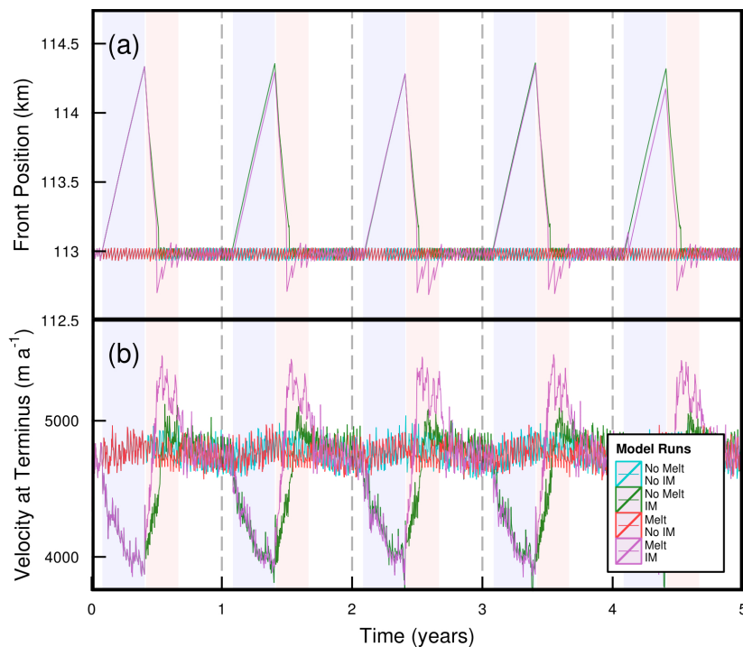
Figure 6. Plots showing changes in calving terminus position (a) and velocity (b) during a five year period within a 40 year long stable simulation, with coloured solid lines illustrating the effect of four different combinations of melting and ice mélange perturbation. Blue and red shade indicates mélange and melt season respectively.
