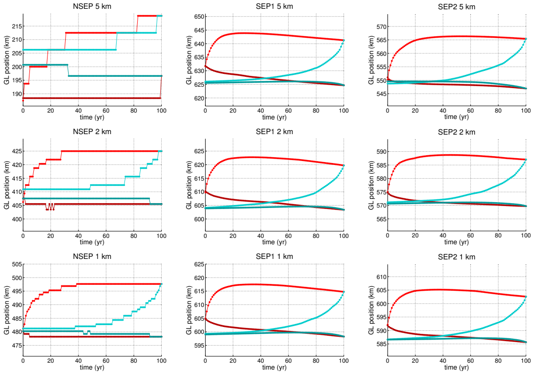
Fig. 5. Time-dependent position of the grounding line along the symmetry axis ( y = 0 ) and the free slip border ( y = 50 ) during (respectively light red and dark red) and after (respectively light teal and dark teal) the friction perturbation for coarse mesh resolutions. y axes have the same scale for all simulations. x axes (time) is after the perturbation experiment (teal lines)
