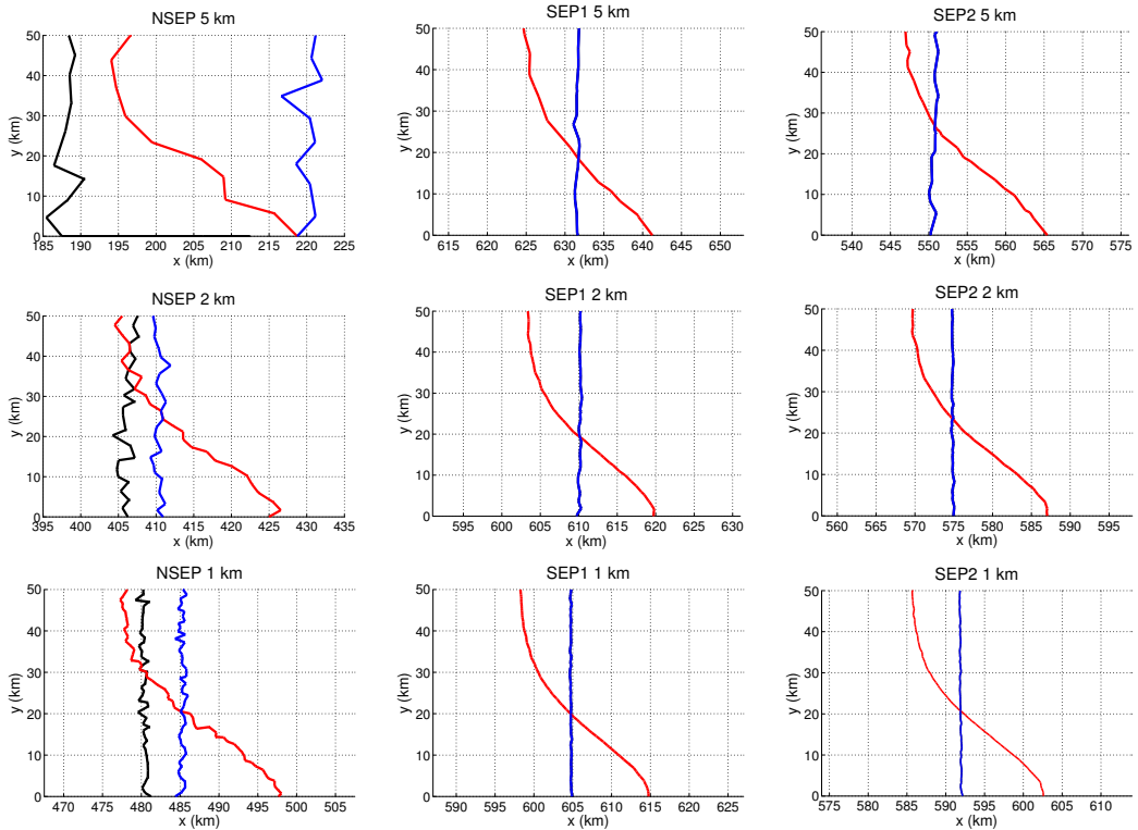
Fig. 3. Initial steady state grounding line positions in the (x, y) plane (black line), position 100 years after the basal perturbation is introduced (red line) and new steady state position after the basal friction is reset to its initial value (blue line). Where black line is not visible, black and blue lines superimpose. x and y axis have the same scale for all plots. results of this experiment: the
