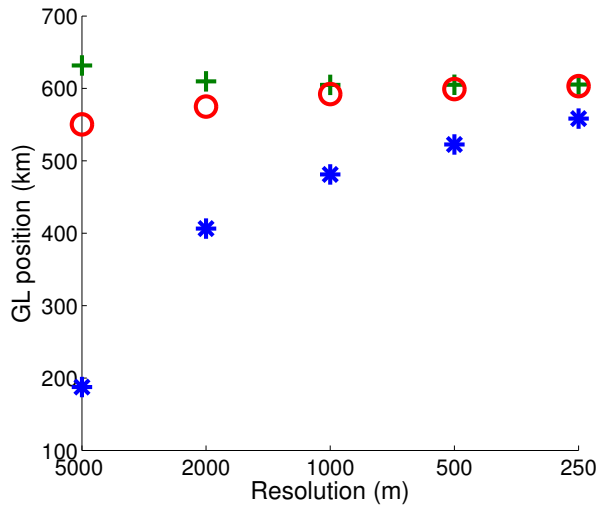
Fig. 2. Steady state grounding line position in y = 0 as a function of mesh refinement for NSEP (blue stars), SEP1 (green crosses) and SEP2 (red circles).
