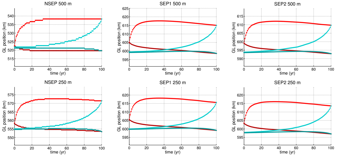
Fig. 6. Time-dependent position of the grounding line along the symmetry axis ( y = 0 ) and the free slip border ( y = 50 ) during (respectively light red and dark red) and after (respectively light teal and dark teal) the friction perturbation for coarse mesh resolutions. y axes have the same scale for all simulations. x axes (time) is after the perturbation experiment (teal lines)
