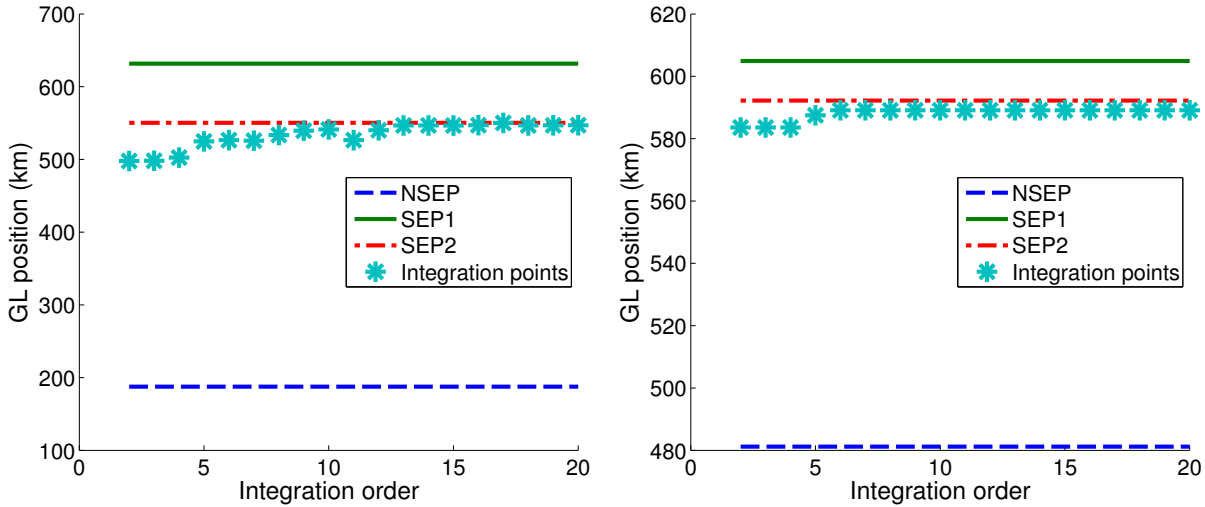
Fig. 7. Grounding line position in y = 0 for 5 km (left) and 1 km (right) resolution mesh for NSEP (dark blue dashed line), SEP1 (green straight line), SEP2 (red dash dotted line) and SEP3 with different integration orders (light blue stars).
