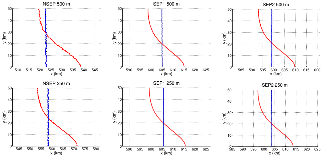
Fig. 4. Initial steady state grounding line positions in the (x,y) plane (black line), position 100 years after the basal perturbation is introduced (red line) and new steady state position after the basal friction is reset to its initial value (blue line). Where black line is not visible, black and blue lines superimpose. x and y axis have the same scale for all plots.
