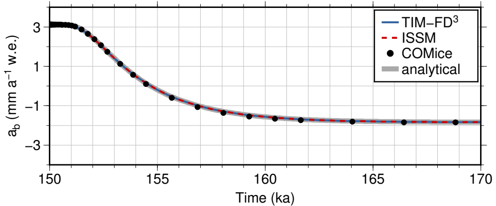
Figure 2. Simulation results compared to the analytical solution (thick solid grey line) for phase IIIa in Experiment A. TIM-FD 3 as blue solid line, ISSM as red dashed line, and COMIce as black filled circles.
