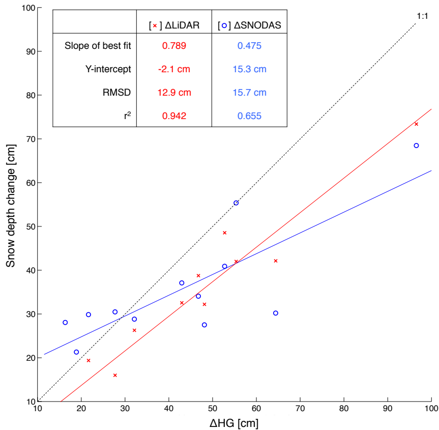
Fig. 4. \Delta SNODAS (blue circles) and \Delta LiDAR (red crosses) snow depths evaluated over the centers of the twelve \Delta HG measurement transects. The \Delta LiDAR points were determined by averaging each reported 5 meter resolution \Delta LiDAR snow depth within a 10 meter radius of each reported HG measurement, then averaging again over each HG transect site. The \Delta SNODAS estimates were the areal-weighted averages of the four nearest SNODAS pixels to the center of each HG transect site.
