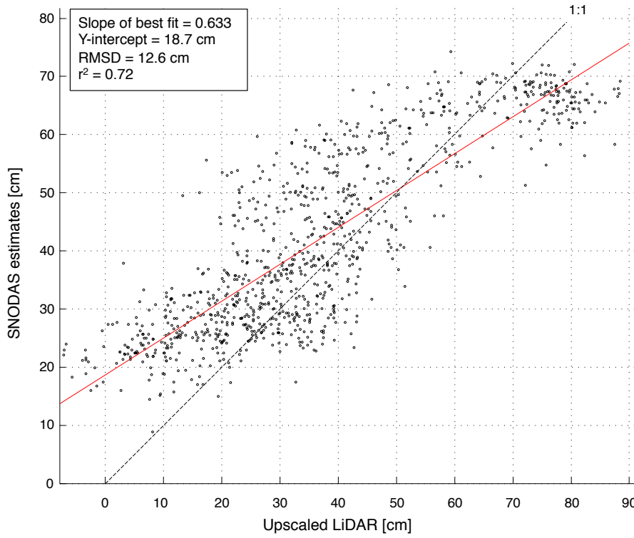
Fig. 5. SNODAS model estimates plotted against mean LiDAR-derived snow depth change within all 1\text{-km}^2 SNODAS pixels ( n=980 ).
