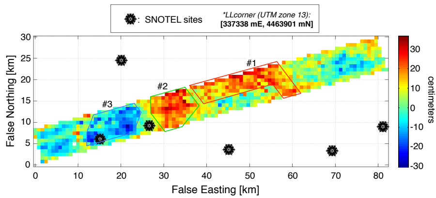
Fig. 7. Image of the difference ( \Delta SNODAS - \Delta LiDAR ) between model and remote sensing estimates of snow depth change between December 3 rd , 2006 and February 22 nd , 2007 over the CLPX-2 study area. The three outlined regions correspond to the regions highlighted in Figure 6.
