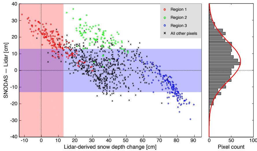
Fig. 6. Pixel by pixel \Delta\text{SNODAS} - \Delta\text{LiDAR} differences of snow depth change plotted against the mean \Delta\text{LiDAR} within each SNODAS pixel. The pink and blue shaded areas represent the \pm 13\text{cm} error threshold for the upscaled LiDAR estimates determined from the CLPX-2 in situ \Delta\text{HG} measurements. Three grouped regions are depicted that were found to contain model pixels of significant \Delta\text{SNODAS} - \Delta\text{LiDAR} discrepancies ( > |\pm 13\text{cm}| ). Also plotted is a histogram of differences showing a bias toward higher SNODAS estimates across the CLPX-2 study area.
