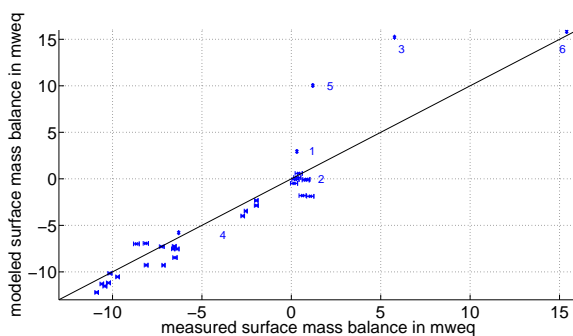
Fig. 3. Comparison between measured and simulated surface mass balance: labels correspond to places marked in Fig. 1. The values in the accumulation area are yearly accumulation values, whilst the ablation data are summer, winter or yearly values depending on the availability of data. The uncertainties of the measurements are indicated as error bars in the x direction if available.
