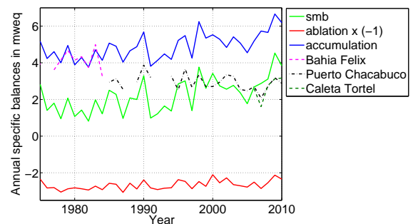
Fig. 4. Annual specific accumulation, ablation and surface mass balance (smb) averaged over the SPI from 1975-2010 and yearly measured precipitation sums for selected weather stations in the region: Bahia Felix ( 52^{\circ}58'S, 74^{\circ}08'W ) south of the SPI, Puerto Chacabuco ( 45^{\circ}26'S, 72^{\circ}49'W ) north of the NPI and Caleta Tortel ( 47^{\circ}47'S, 73^{\circ}32'W ) between NPI and SPI.
