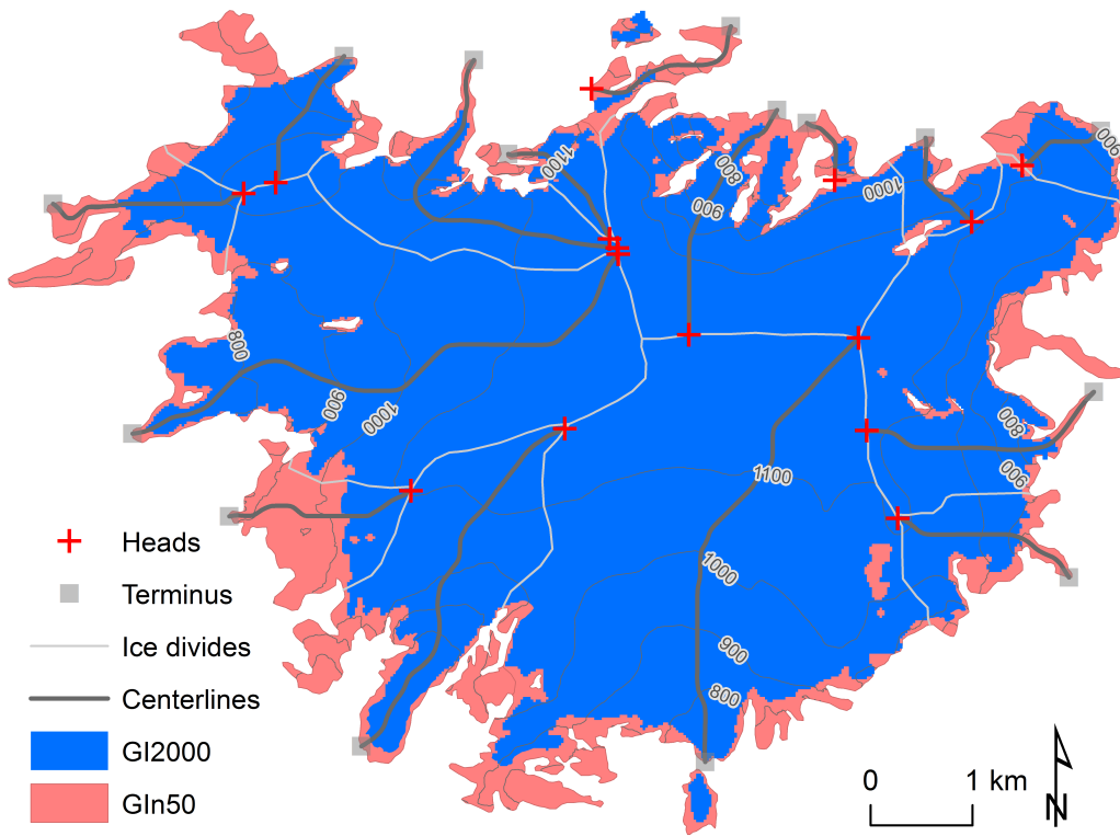
Figure 4. GI 50 and GI 2000 presented with the automatic derived glacier heads, termini and centerlines at Øksfjordjøkelen.
