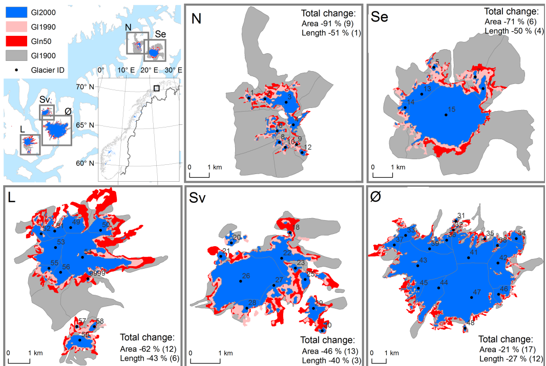
Figure 8. Glacier area and length change for five ice caps in West-Finnmark. The numbers after the mean percentage area and length change are the number of included glacier units (area) or centerlines (length). N = Nordmannsjøkelen, Se = Seilandsjøkelen, L = Langfjordjøkelen, Sv = Svartfjelljøkelen, and Ø = Øksfjordjøkelen.
