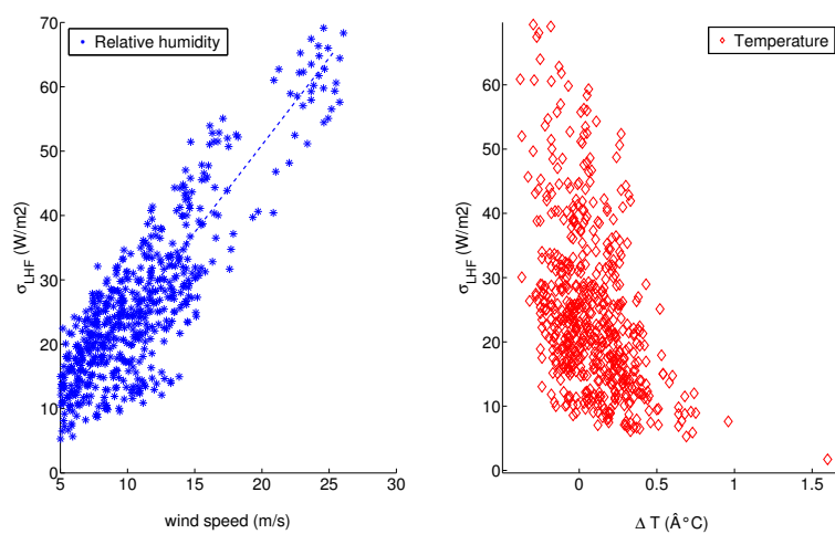
Fig. 12. Uncertainty propagation into the latent heat flux from measurements uncertainties via profile calculations.
