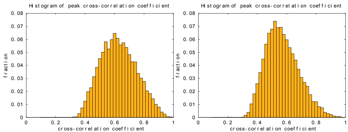
Fig. 15. Maximum cross-correlation coefficient histogram for the A1-A2 image pair (L-L), left, and the A1-E2 image pair (L-C), right.
