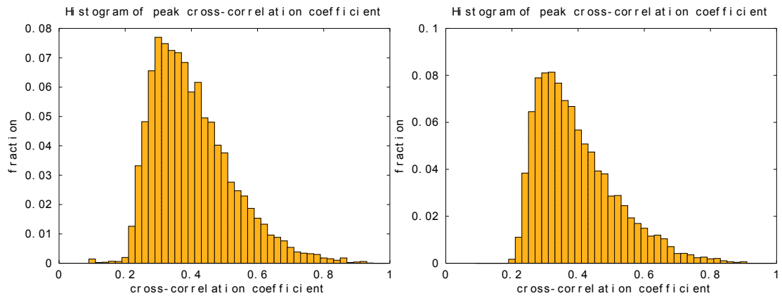
Fig. 14. Maximum cross-correlation for matched windows in the R2-A2 image pair (C-L, left) and the R2-E2 image pair (C-C, right)
