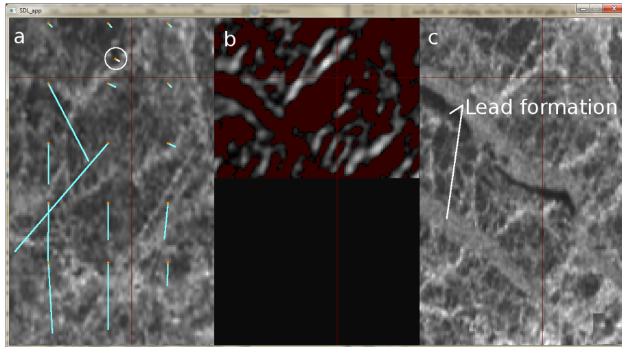
Fig. 4. Screenshot of the motion estimation program written for this work. a) zoom-in of the first image with some detected motion vectors. b) the cross-correlation result for the circled vector. White represents maximum cross-correlation, black represents zero correlation and the area left outside of the calculation. Red represents negative cross-correlation. c) aligned zoom-in of the second image of the pair. Notice the newly formed NW-SE aligned leads. The thin red lines are rulers that highlight the mouse cursor's location.
