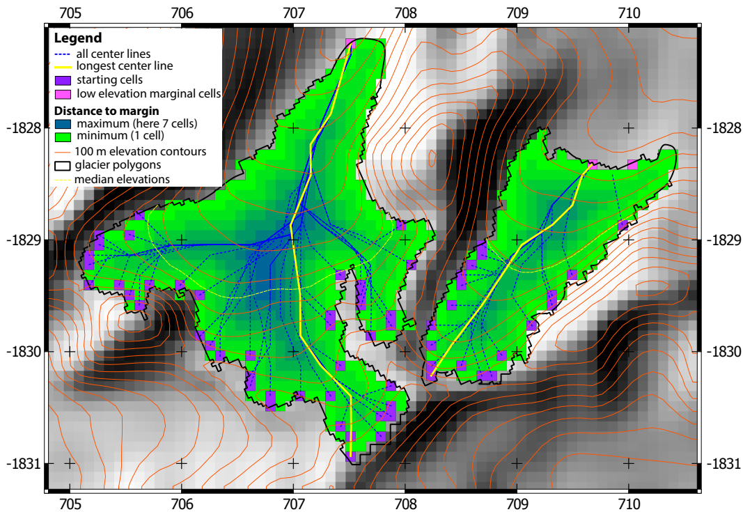
Fig. 3. All calculated center lines including the selected longest center lines calculated for two small mountain glaciers of East Greenland. Coordinates as in Fig. 2.
