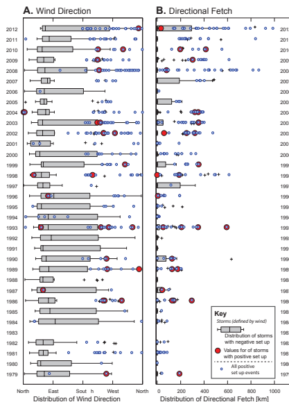
Figure 15. Wind direction (A) and directional fetch (B) by year for all storms (defined as wind \geq 10 \text{ m s}^{-1} ) and for positive set up events. Storms that set up water and positive set up events have winds from the west and north. Directional fetch during storms that set down water and positive set up events has increased through time while directional fetch during storms that set up water does not exhibit this trend.
