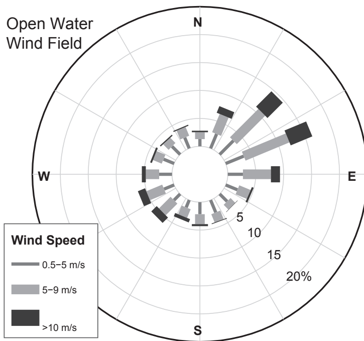
Figure 3. Wind field at Drew Point during both the sea ice (A) and the open-water season (B). The wind field is dominated by wind from the ENE but show a smaller secondary maximum from the WSW (data from Urban and Clow, 2013).
