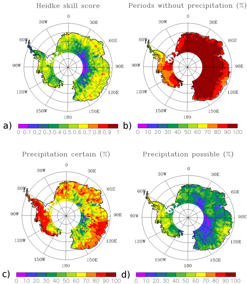
Fig. 4. Comparison between the precipitation samples from CloudSat and ERA Interim reanalysis for the period August 2006 - April 2011. In ERA Interim reanalysis, precipitation events were defined for a precipitation rate over 0.07 mm / 6 h. a) Heidke Skill Score assessed using samples indicating precipitation certain and period without precipitation. b) Proportion of samples indicating periods without precipitation that match with periods without precipitation in ERA Interim. c) Proportion of samples indicating precipitation certain that match with precipitation events in ERA Interim. d) Proportion of samples indicating precipitation possible that match with precipitation events in ERA Interim.
