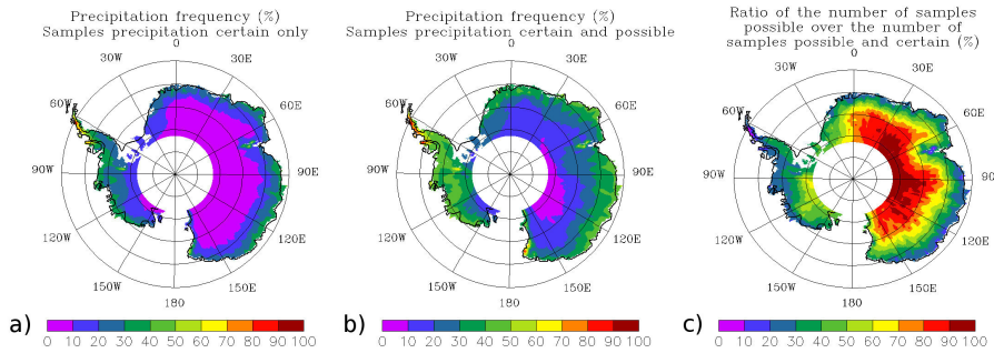
Fig. 2. a) Precipitation frequency (%) with the samples indicating precipitation certain for the period August 2006 - April 2011. b) Precipitation frequency (%) with the samples indicating precipitation certain and possible for the period August 2006 - April 2011. c) Ratio of the number of samples indicating precipitation possible over the number of samples indicating precipitation certain and possible.
