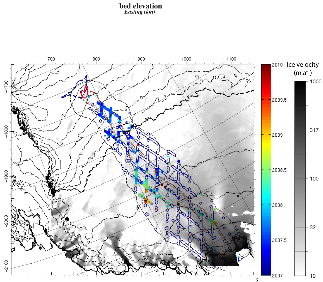
Figure R2. Figure 5 superimposed onto a map of ice surface velocity (Rignot et al., 2011).
