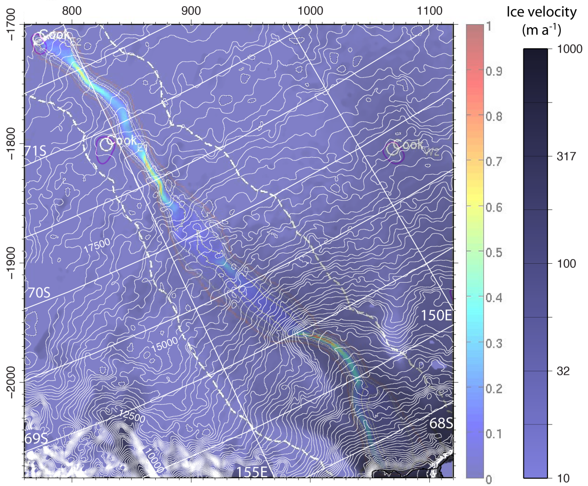
Figure R1. Figure 4 with hydropotential based on the Bedmap 2 dataset for ice surface topography and ice thickness (Fretwell et al., 2013).
