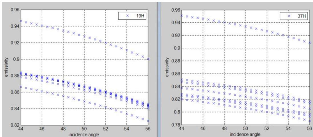
Fig. 1. 19H and 37H emissivities vs. incidence angle
