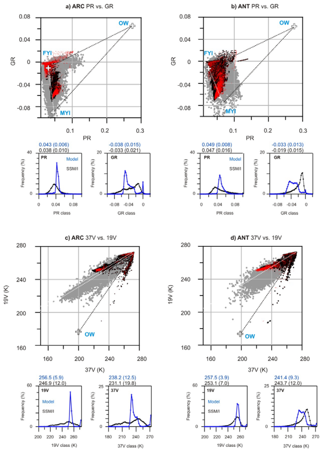
665 Figure 2. Simulated brightness temperatures polarization and gradient ratios (PR, GR, black) for the Arctic (a, January to June) and Antarctic (b, July to December) and brightness temperatures at 37V/19V for the Arctic (c) and Antarctic (d), 4 times daily data, 2000-2009. Red dots indicate last month of simulations. Daily values of observed satellite Tb for area with sea-ice concentrations above 90% are shown by grey dots for comparison. Tie points for open water (OW) and (a, b only) first-year ice (FYI) as well as multi-year ice (MYI) are
