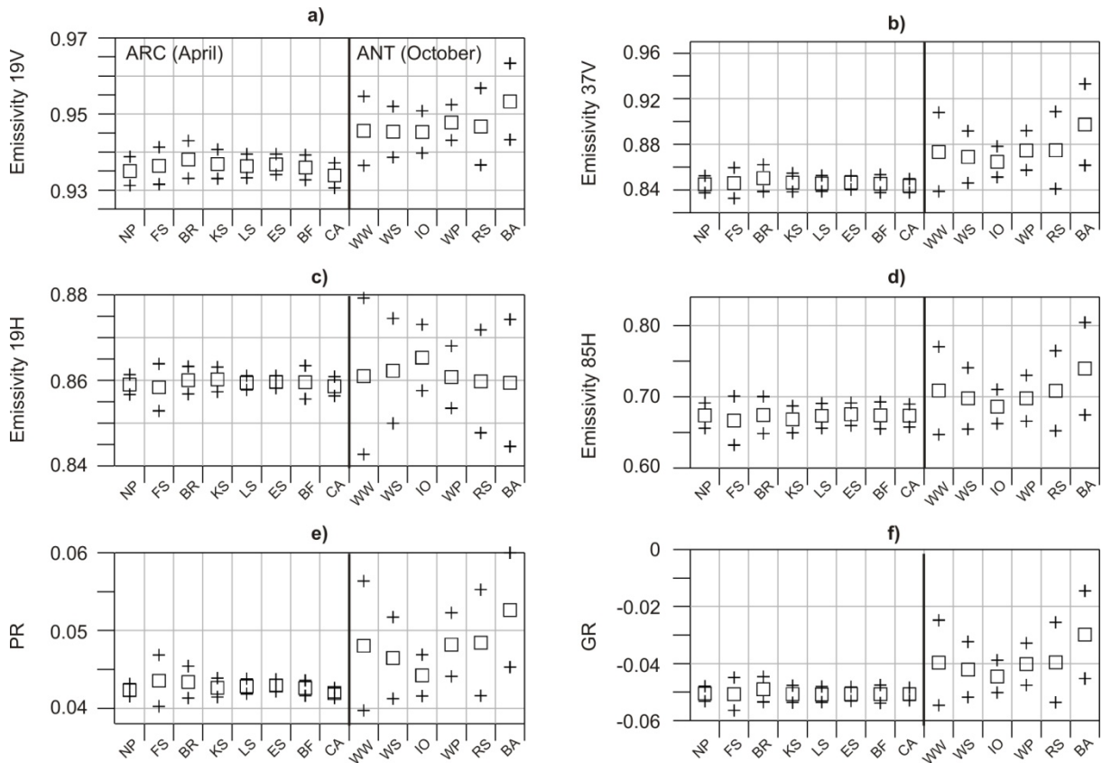
Figure 5. Mean (squares) and standard deviation (crosses) of simulated emissivity values indicating the daily, spatial and interannual variability in the 4th month of simulation (ARC: April, ANT: October) for emissivities at a) 19V, b) 37V, c) 19H, d) 85H as well as e) Polarization Ratio and f) Gradient Ratio.
